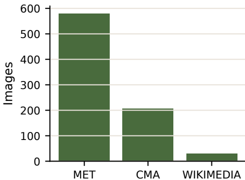
Source distribution
