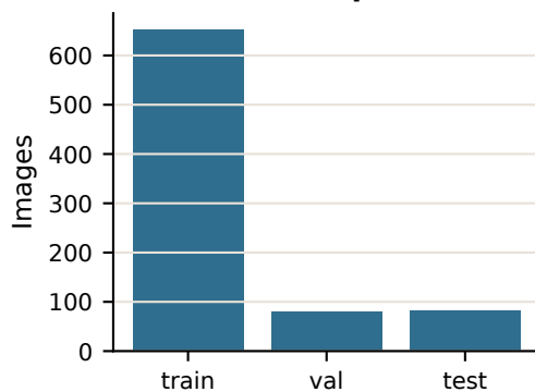
Data split
