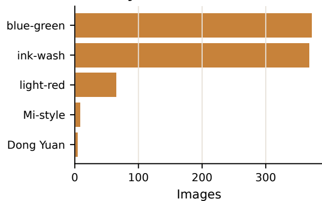
Style-label distribution
