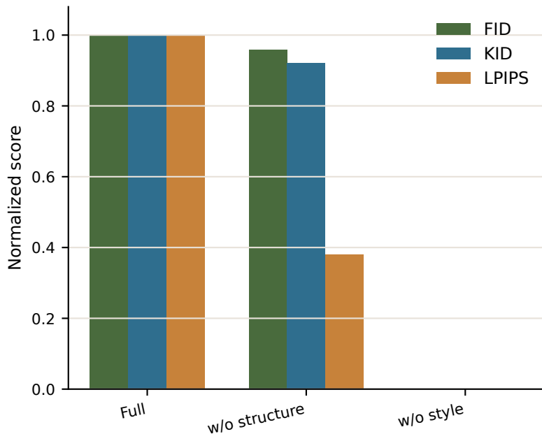
Pilot component ablation
