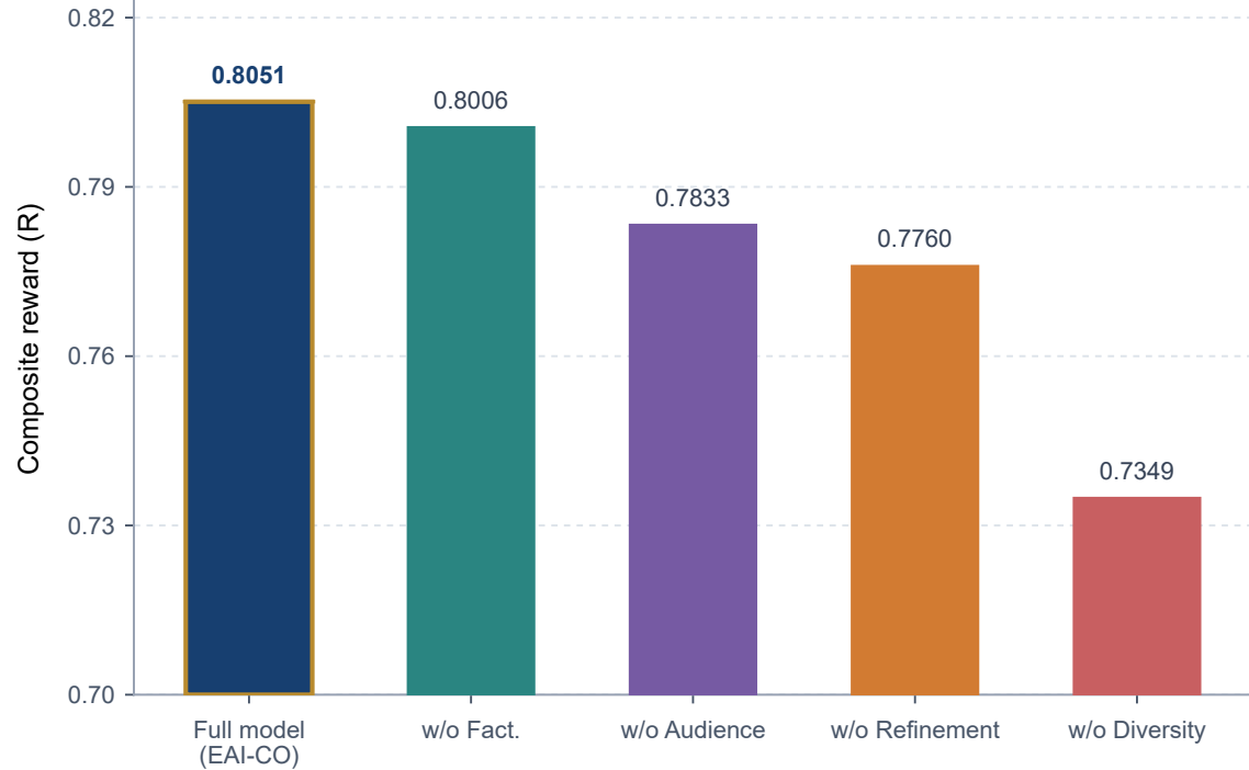
Absolute performance
