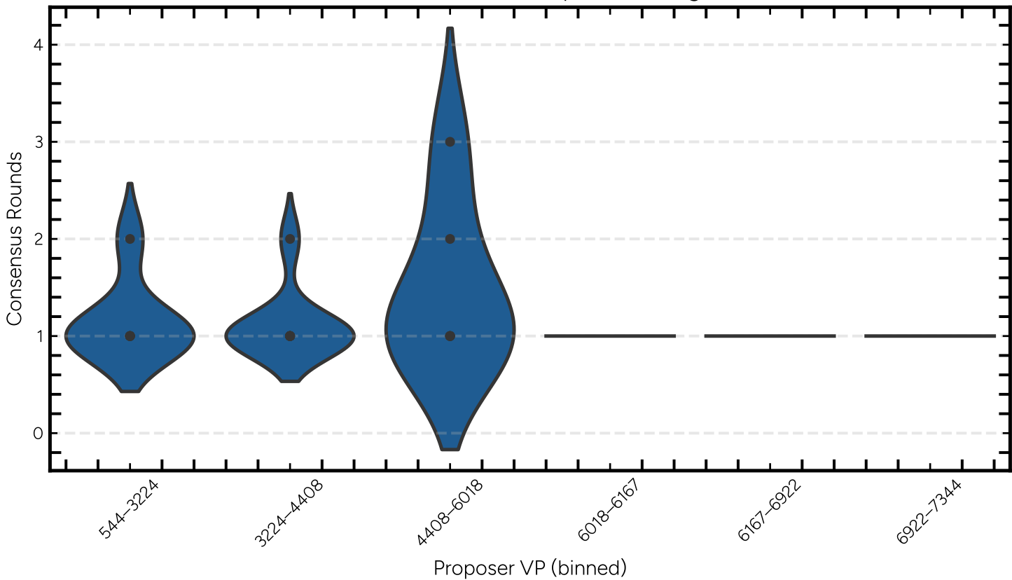
Consensus Rounds vs Proposer Voting Power
