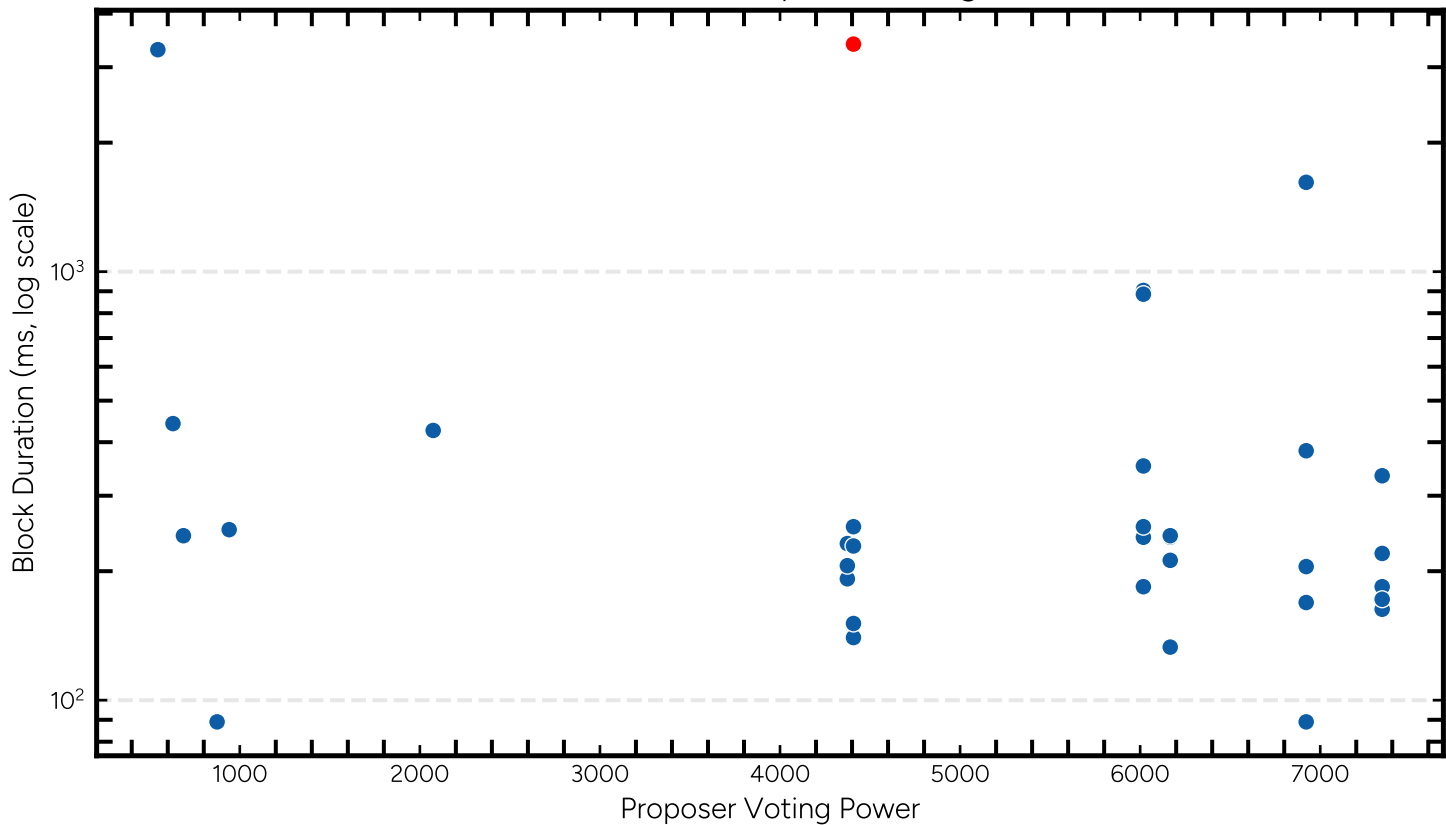
Block Duration vs Proposer Voting Power
