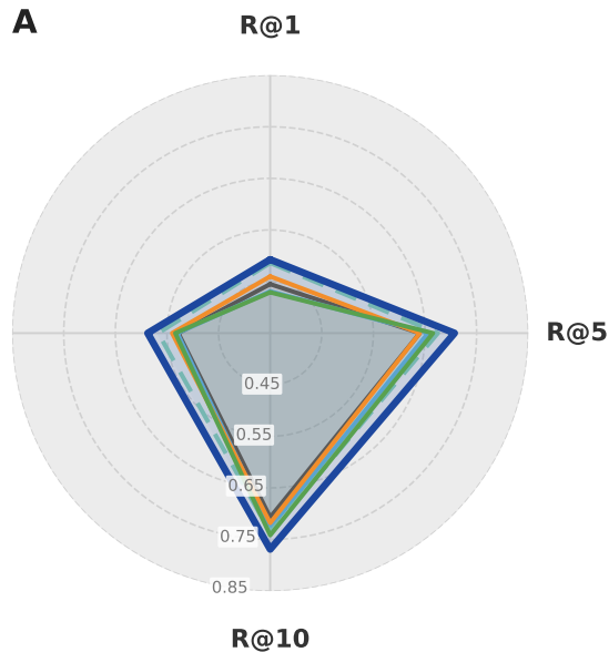
Task 1 — CVE Linkage Retrieval
