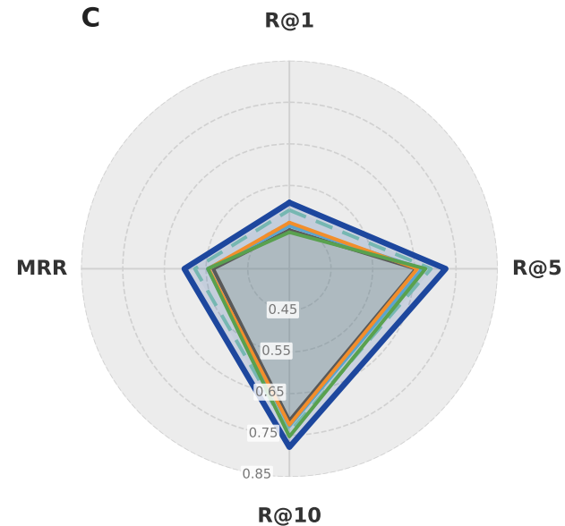
Task 3 — Temporal Generalization
