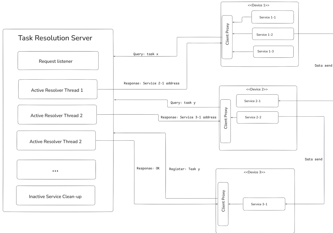
Figure 2: Client machines operating in server architecture
