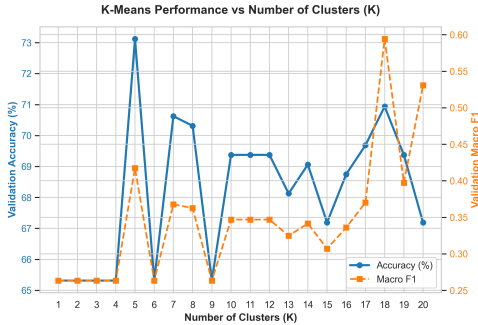
Figure 2: K-Means validation scores vs. K
