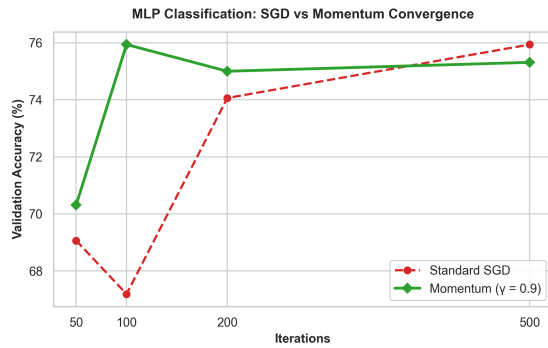
Figure 2: MLP Classification: SGD vs Momentum Validation Accuracy
