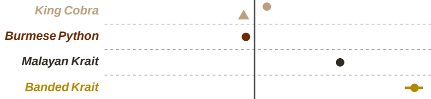
Binary Habitat Classification
