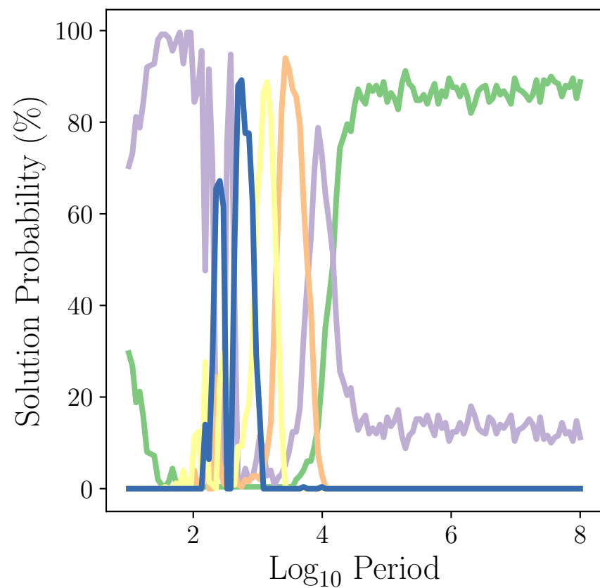
Circular Orbits
