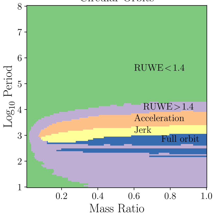
Circular Orbits
