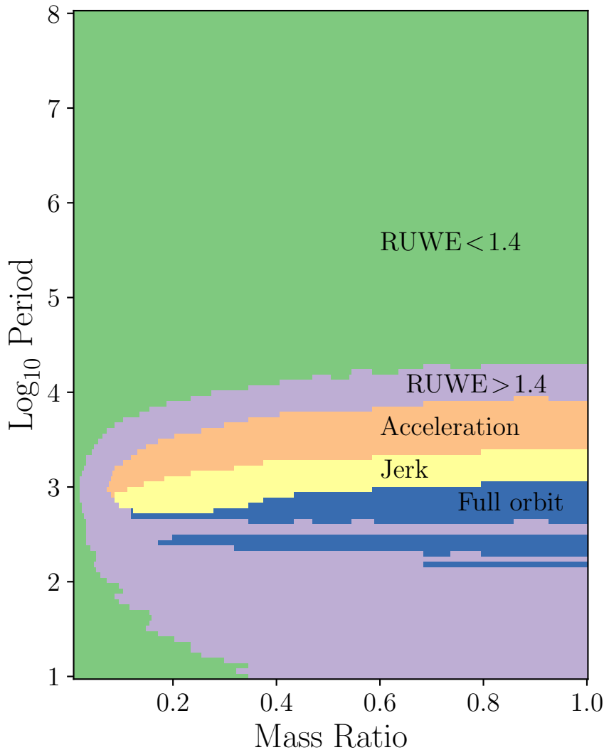
Circular Orbits
