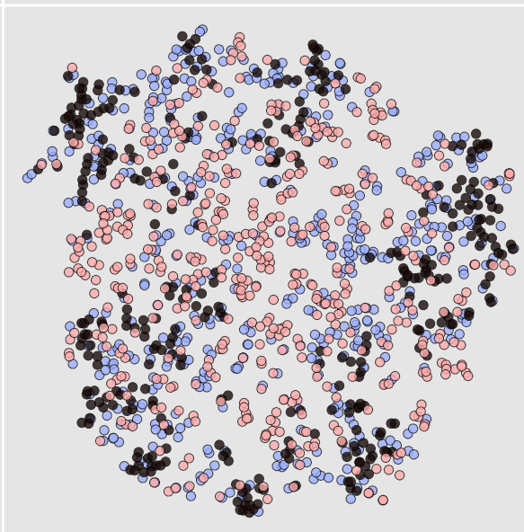
Residual (per Qubit)
