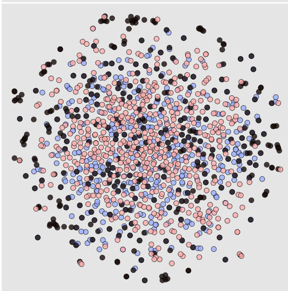
Log Ratio
