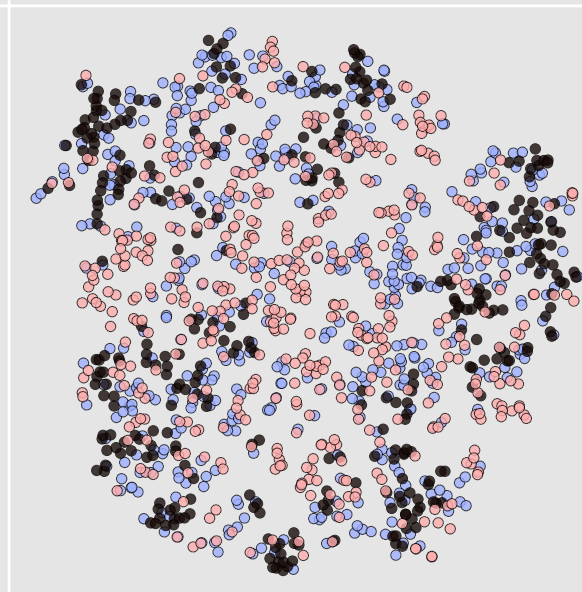
Pauli-Z Expectation
