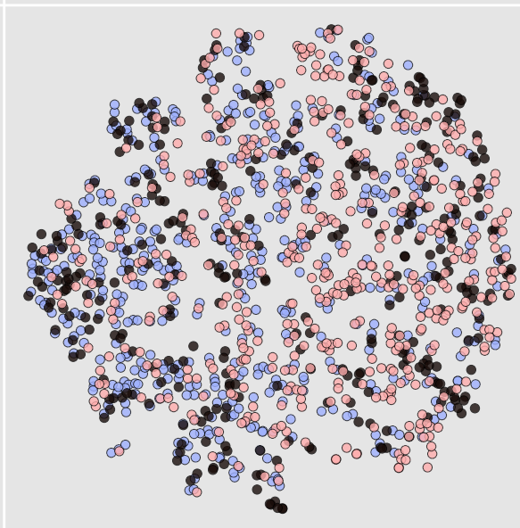
Residual (Absolute, per Qubit)
