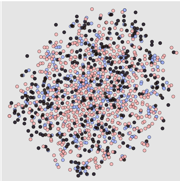
Residual
