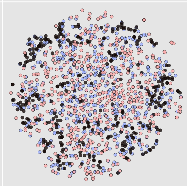
Two-Qubit Correlator
