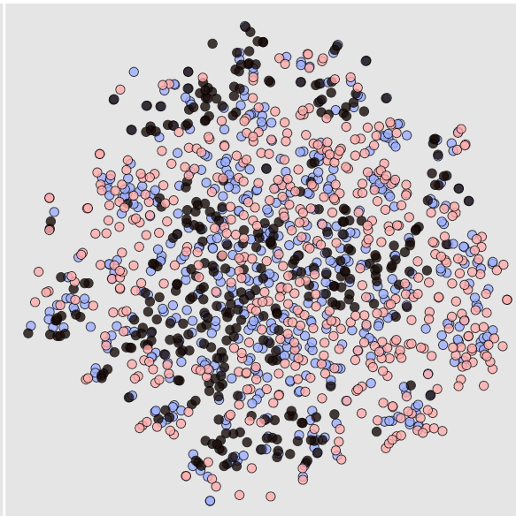
Residual (Absolute)
