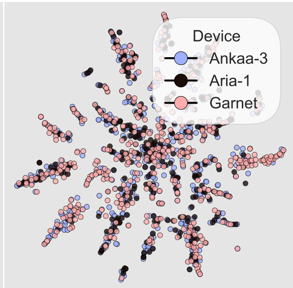
Residual (Absolute, Relative)
