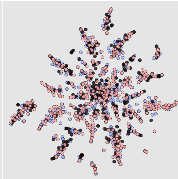
Residual (Relative)
