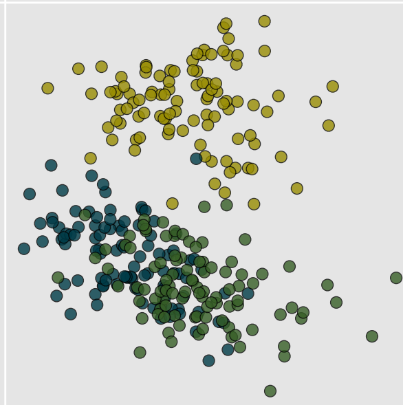
Residual (Absolute, per Qubit) (Var: 0.928)
