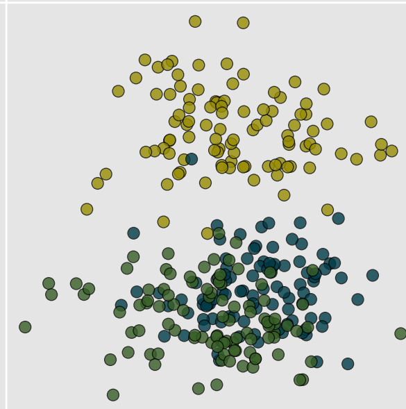
Pauli-Z Expectation (Var: 0.851)
