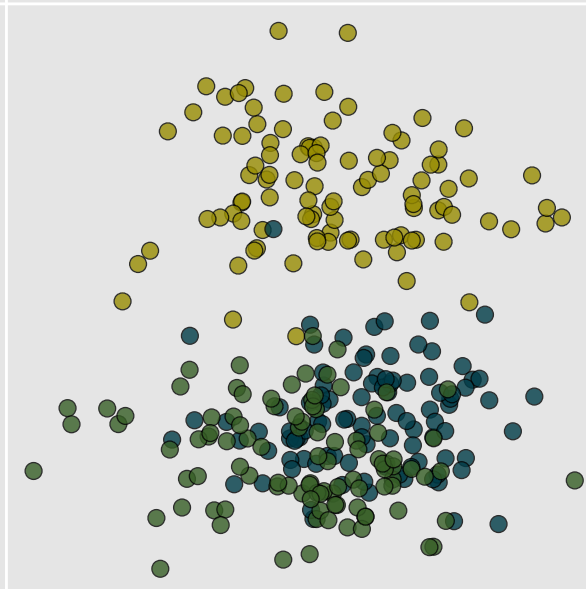
Residual (per Qubit) (Var: 0.851)
