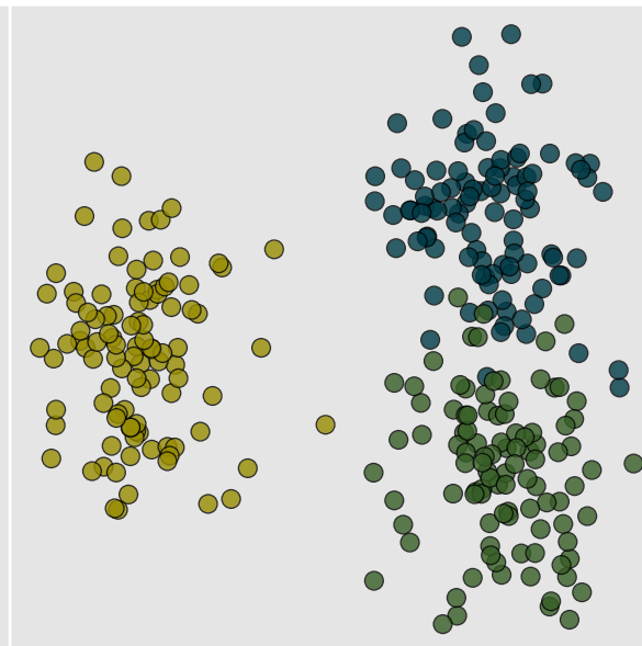
Residual (Relative) (Var: 0.286)
