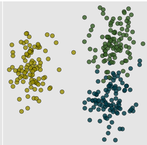
Residual (Absolute, Relative) (Var: 0.286)
