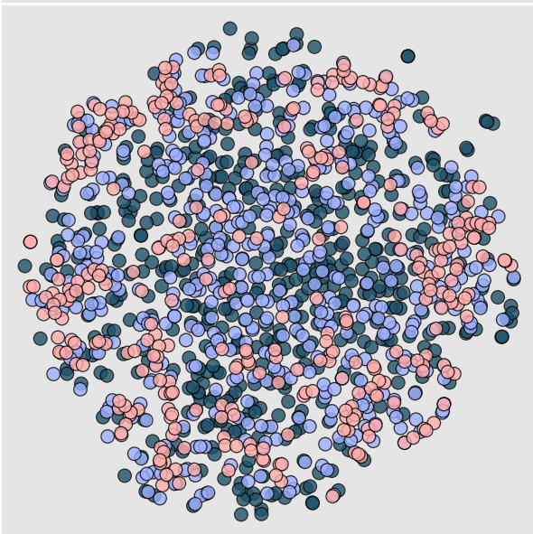
Two-Qubit Correlator
