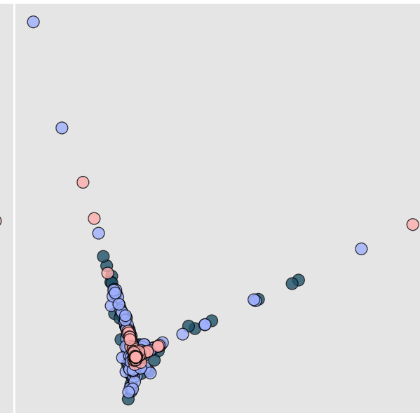
Residual (Absolute, Relative) (Var: 0.071)
