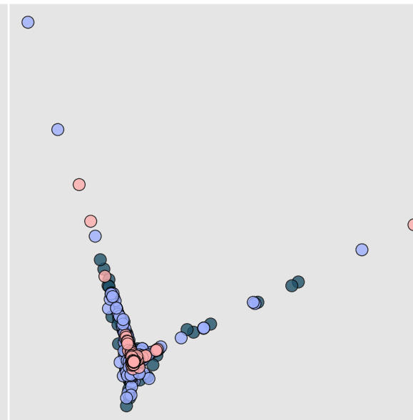
Residual (Relative) (Var: 0.071)
