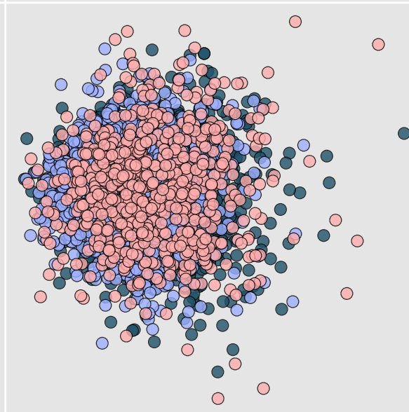
Residual (Absolute, per Qubit) (Var: 0.685)
