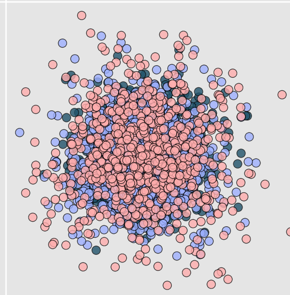
Pauli-Z Expectation (Var: 0.507)
