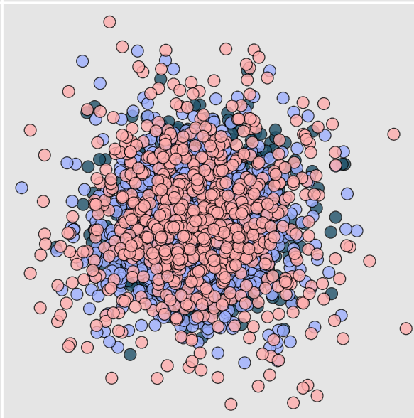
Residual (per Qubit) (Var: 0.507)
