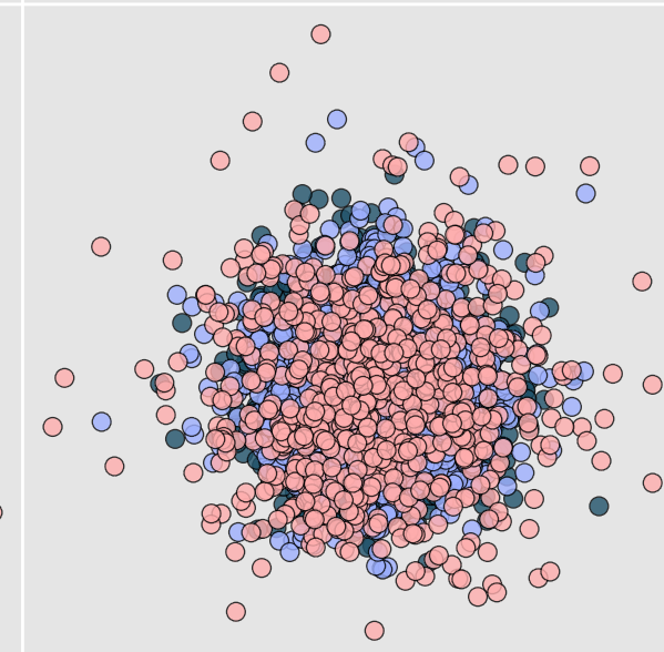
Two-Qubit Correlator (Var: 0.247)
