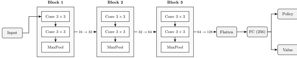
Figure 2.1: The IMPALA encoder architecture. Each block contains two 3 \times 3 convolutions followed by max-pooling. Channel counts double between blocks ( 16 \rightarrow 32 \rightarrow 64 \rightarrow 128 ). The flattened output feeds into a fully-connected layer producing a 256-dimensional embedding, which is then split into policy and value heads.
