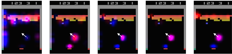
Figure 2.4: Saliency maps for a DQN agent learning to play Breakout, showing the evolution of attention patterns during training. Blue regions indicate areas most salient to the actor (policy), while red indicates areas salient to the critic (value function). Early in training, attention is diffuse; as learning progresses, the agent focuses on strategically relevant features such as the ball and the tunnel through the brick wall. Figure reproduced from Greydanus et al. (2018).
