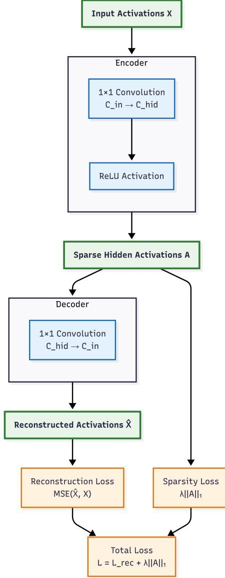
Figure 2.3: Sparse auto-encoder (SAE) architecture. An encoder applies a 1 \times 1 convolution and ReLU to map input activations X to sparse hidden activations A ; a second 1 \times 1 convolution reconstructs \hat{X} . Training minimises the reconstruction loss \text{MSE}(X, \hat{X}) plus an \ell_1 sparsity penalty \lambda \|A\|_1 . Shapes: X \in \mathbb{R}^{B \times C_{\text{in}} \times H \times W} , A \in \mathbb{R}^{B \times C_{\text{hid}} \times H \times W} , \hat{X} \in \mathbb{R}^{B \times C_{\text{in}} \times H \times W} .
