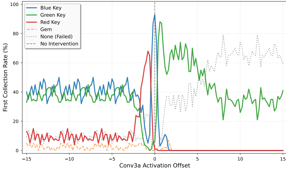
Figure 2: Full range activation offset sweep for conv3a layer at checkpoint 35001. Each subplot shows entity collection success rates across different activation offset values for a specific channel. This wide-range sweep reveals the broad activation ranges over which different channels can successfully steer the agent toward specific entities.
