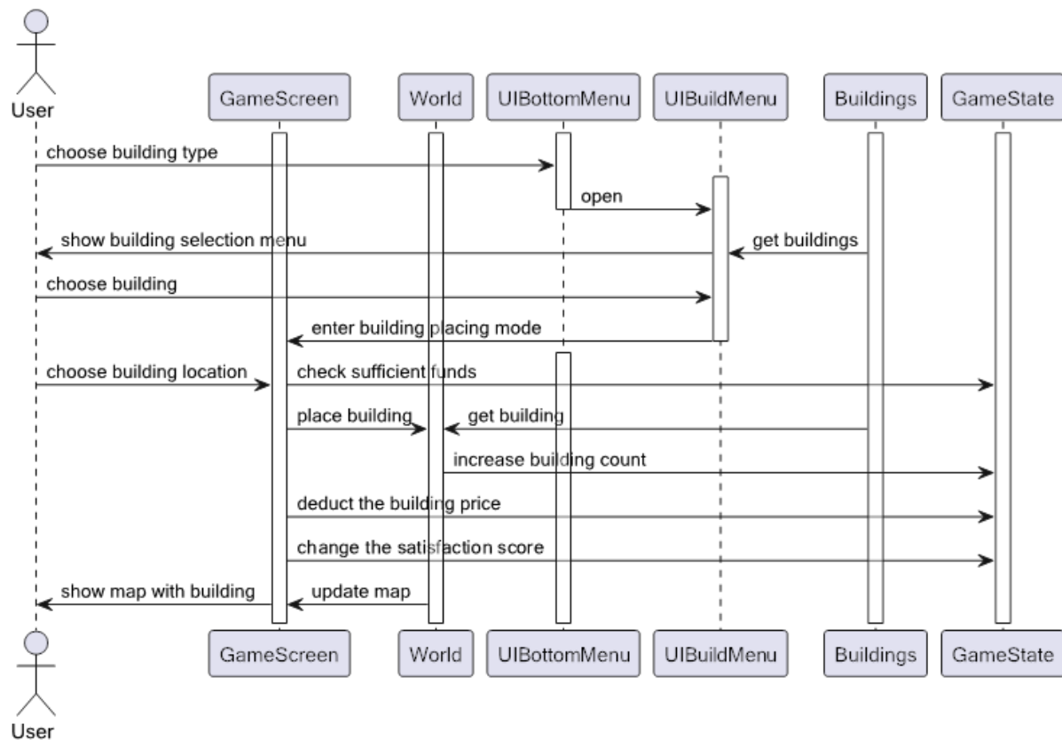
Figure 2: A UML sequence diagram showcasing the building placement use case.
