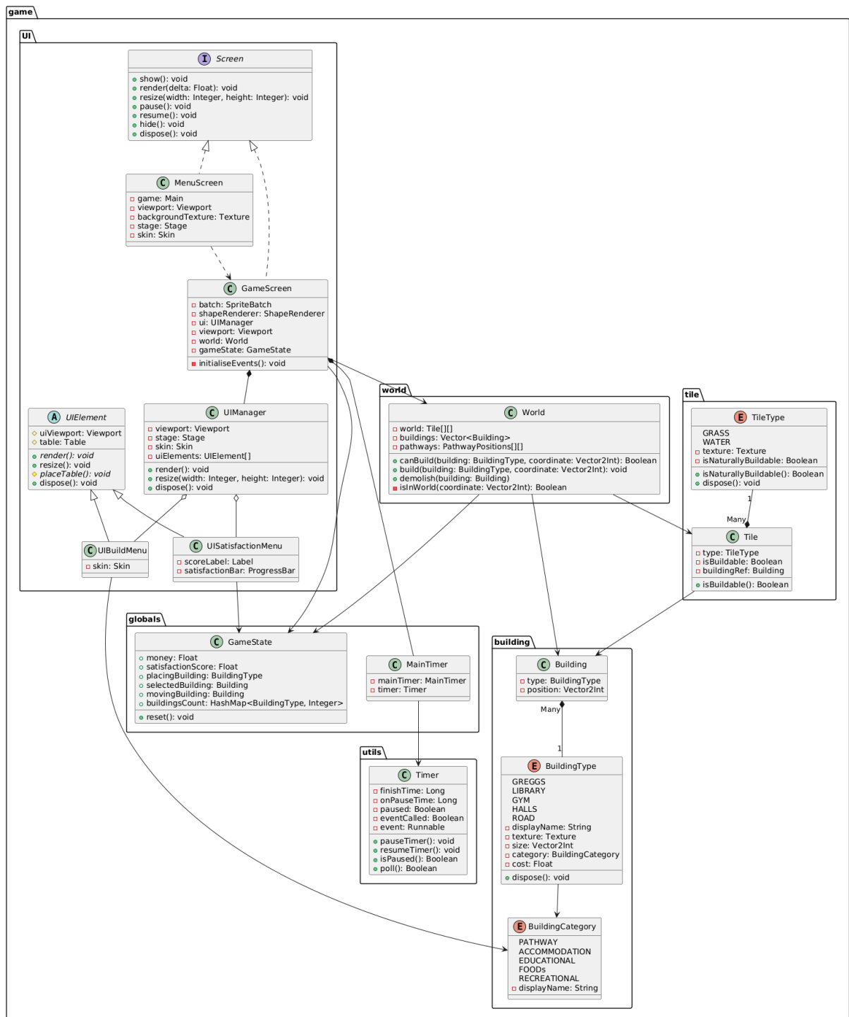
Figure 1: An extensive UML diagram constructed with plantUML [1] depicting the relations at the end of stage 1.
