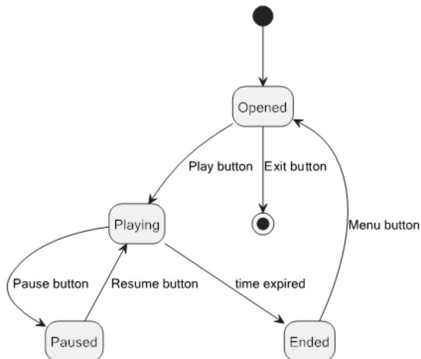
Figure 3 : A UML state diagram showcasing interactions within the game that alter its states.
