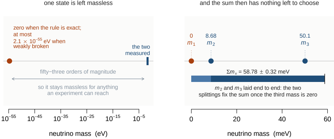
Figure 13: What the rule does to the spectrum. Left, the full range. When the rule is exact the sterile partner’s Yukawa column is forbidden, the light mass matrix has rank at most two, and one light neutrino is exactly massless; the weakly broken version below lifts that zero to at most 2.1 \times 10^{-55} eV for the example lifetime, fifty-three orders of magnitude below the lighter of the two measured splittings. Right, the same spectrum on a linear scale in meV. With m_1 at zero the two splittings fix the sum with nothing left to choose, \Sigma m_\nu = \sqrt{\Delta m_{21}^2} + \sqrt{\Delta m_{31}^2} = 58.78 \pm 0.32 meV for normal ordering, drawn as the two masses laid end to end.
