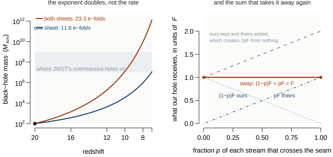
Figure 10: What a second supply would have given, and the ledger that removes it. Left: growth from a 100 M_{\odot} seed between z = 20 and z = 7 , Eddington-limited at radiative efficiency 0.1. A supply multiplier does not add to the mass, it multiplies the exponent, so 11.6 e-folds become 23.3 and the final hole is 10^5 times heavier. That is the prize, and it is why the section checked rather than adopted. Right: the two-channel ledger that forbids it. Fold invariance makes the two sheets' infall equal, and a crossing inside the contact radius is a swap, so our hole receives (1-p)F of our own stream and pF of theirs for a total of F at every p . The alternative, keeping our own and adding theirs, is the dashed line, and it creates 2pF from nothing.
