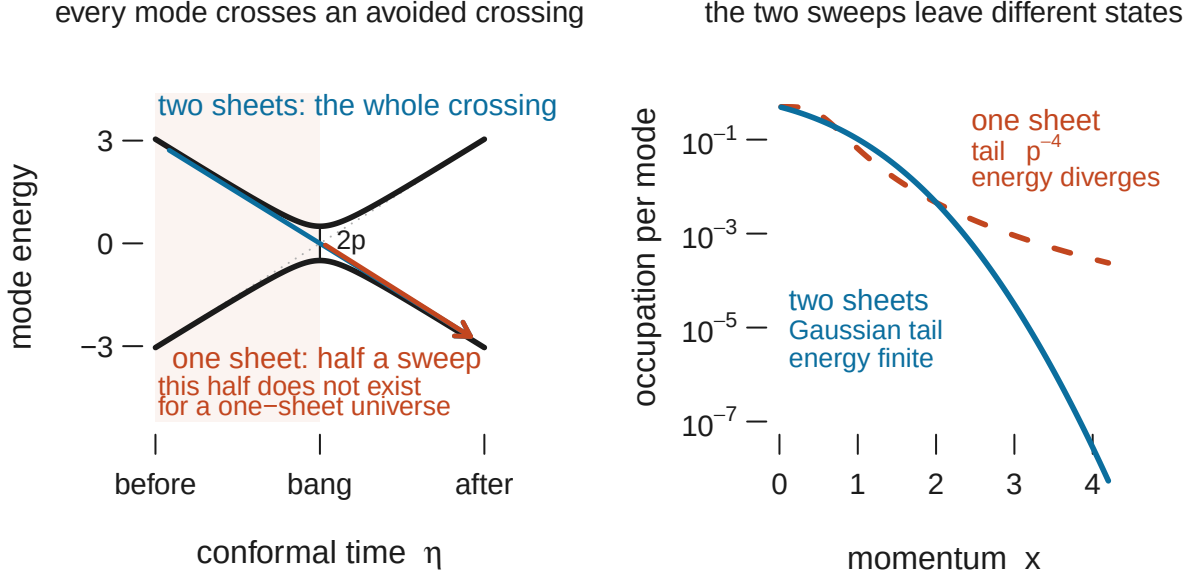
Figure 1. Every mode at a radiation bang passes through an avoided crossing; the gap at closest approach is 2p . A universe with one sheet begins at the bang and gets half the sweep. A universe with two runs the whole way through. The right panel is what each leaves behind: the half sweep produces a p^{-4} occupation tail whose energy integral diverges logarithmically, and the whole crossing produces the Gaussian the observed abundance needs. Both curves are the closed forms, and the one-sheet curve is drawn as an illustrative profile with the stated tail index rather than a particular state.
