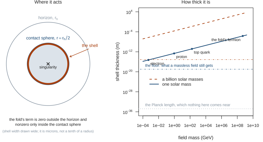
Figure 4. Where the fold leaves general relativity, and how thick that place is. Left: the fold's extra term is suppressed to nothing measurable outside the horizon and acts only inside the contact sphere at r = r_h/2 , and the shell drawn in at the edge of that region is where it is the larger of the two terms acting on an infalling congruence. The shell is drawn wide to be visible; it is microns, not a tenth of a radius. Right: that thickness against the field's mass, at one solar mass and at a billion, with the Planck length marked. Nothing on the plot comes near it, which is the result: the departure is a real length for every field there is. The two dashed horizontals are the floor the mass-independent part of the same stress leaves, 1.1 \times 10^{-19} m and 7.8 \times 10^{-16} m, which the sloping curves meet only for a field lighter than anything in the Standard Model and below which nothing goes. Both curves are D_*/r_h = (8\pi\kappa(m/m_P)^2/11.5138)^{2/5} with \kappa = 0.0039 , recomputed in the figure's own code and asserted against the file that supplies the coefficient.
