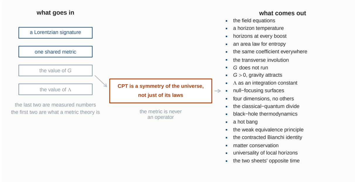
Figure 5. The ledger. On the left is everything the fold is given: a Lorentzian signature and one metric carrying both the fold's horizons and a covariant matter action, which between them are what writing a metric theory means, and the measured values of G and \Lambda . In the middle is the single postulate, that CPT is a symmetry of the universe and not only of its laws. On the right are the nineteen properties of general relativity that follow, the metric staying a fixed background throughout. The dependency graph behind the two columns is acyclic and no path from the field equations reaches general relativity or Bekenstein-Hawking entropy, which is what stops the argument assuming its own conclusion. The labels are the ledger's own lines and their counts are read from it, so the figure cannot drift from the text, and Appendix E gives the same lines at full wording. What the figure does not draw, because it is not a property of general relativity, is the Hadamard condition on states, which §4.1 names as the sixth root of the dependency graph.
