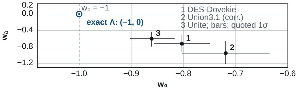
Figure 3. Neutrino mass and dark-energy context. (a) The massless-lightest-neutrino markers in the exact stabilising-rule sector at 58.8 meV (normal ordering, m_1 = 0 ) and 100.9 meV (inverted, m_3 = 0 ), against DESI DR2 BAO + CMB bounds from Elbers et al. [12]: 64.2 meV for \Lambda CDM, the cold-dark-matter cosmology with a constant \Lambda , and 163 meV for w_0w_a CDM, the same with dark energy allowed to evolve, and the 53 meV
