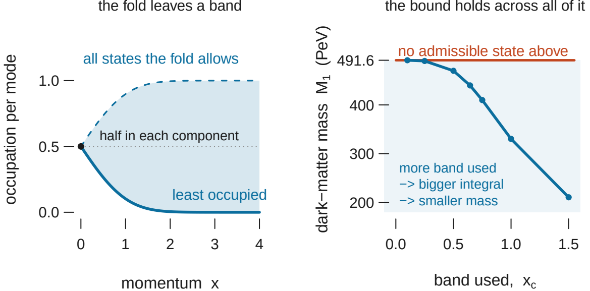
Figure 2. Why the mass is a ceiling. Left: \Theta -invariance forces every mode half into each component at the bang, so the band of allowed occupations has zero width in the deep infrared and opens with momentum; the solid curve is the least-occupied member and the dashed one its particle-hole conjugate. Right: the mass each member of the family returns. Every excursion into the band raises the production integral, and M_1 falls as I^{-2/5} , so the least-occupied member sits at the top.
