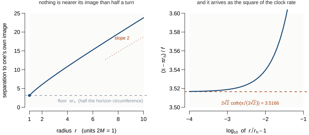
Figure 8: How far a point is from its own fold image. Left: the separation across the exterior on the t = 0 slice, against the floor \pi r_h that the angular half-turn requires and which nothing on that slice goes below. Far from the hole the curve runs at slope two, because leaving the hole moves a point away from its image twice over. Right: the approach to the floor divided by f = 1 - r_h/r , the square of the local clock rate, flattening onto 2\sqrt{2} \coth(\pi/(2\sqrt{2})) = 3.5166 . The two integrals are redone in R for the figure and reproduce the values quoted here to four decimals, which makes the figure a check on its own numbers as well as a picture of them.
