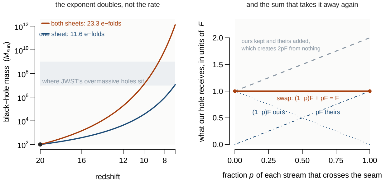
Figure 9: What a second supply would have given, and the ledger that removes it. Left: growth from a 100 M_{\odot} seed between z = 20 and z = 7 , Eddington-limited at radiative efficiency 0.1. A supply multiplier does not add to the mass, it multiplies the exponent, so 11.6 e-folds become 23.3 and the final hole is 10^5 times heavier. That is the prize, and it is why the section checked rather than adopted. Right: the two-channel ledger that forbids it. Fold invariance makes the two sheets' infall equal, and a crossing inside the contact radius is a swap, so our hole receives (1 - p)F of our own stream and pF of theirs for a total of F at every p . The alternative, keeping our own and adding theirs, is the dashed line, and it creates 2pF from nothing.
