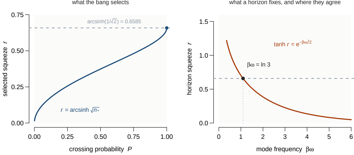
Figure 13: The two ends of the fold, and the one frequency where they agree. Left: what the crossing at the bang selects. Fold-invariance forces half-and-half occupancy, so the pair-block floor is n_*(P) = (1 - \sqrt{1 - P})/2 , and since a squeeze carries \langle N \rangle = \sinh^2 r the selected occupation is a selected squeeze r = \operatorname{arcsinh} \sqrt{n_*} , topping out at \operatorname{arcsinh}(1/\sqrt{2}) = 0.6585 when the crossing is complete. Right: what equilibrium at a bifurcate horizon fixes, the half-period shift making the state a thermofield double with \tanh r = e^{-\beta\omega/2} . The dashed line is the same in both panels, and the horizon curve crosses it at \beta\omega = \ln 3 exactly, to machine zero. The reason is that both ends are statements about one half: \Theta -invariance caps the crossing at half occupancy, a horizon mode is half occupied where the Bose factor is one half, and that is e^{\beta\omega} = 3 . The curves meet because they say the same thing.
