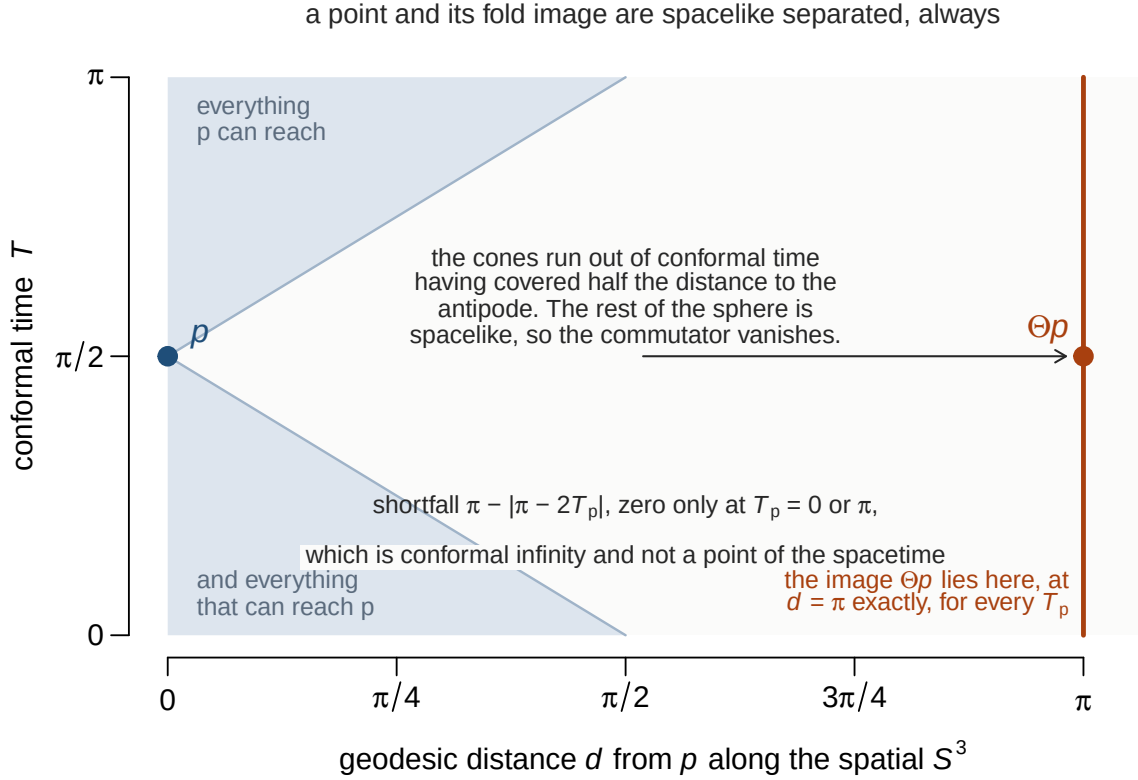
Figure 1: Why. de Sitter is conformal to a piece of the Einstein static cylinder, with round three-spheres for spatial slices and a conformal time running over an interval of length \pi . The antipodal map of the embedding is the antipodal map of that S^3 together with T \mapsto \pi - T , and two points antipodal on a sphere are at geodesic distance \pi whatever their position, so the image of p sits on the right-hand edge at every conformal time. The horizontal axis is therefore distance along S^3 rather than the polar angle, because the conformal square hides the angular part of the separation and that part is the whole argument. Radial null rays are then lines at forty-five degrees, and both of p 's cones run out of conformal time having covered less than half of the way round: the future one at T = \pi and the past one at T = 0 . The shortfall is \pi - |\pi - 2T_p| , which is positive for every point of the spacetime and reaches zero only at conformal infinity. Equivalently and with no picture, Z = X \cdot Y / \ell^2 is one at coincidence and exceeds one for timelike separation, and Z(X, -X) = -1 . A map turning through only half as much of the sphere fails this.
