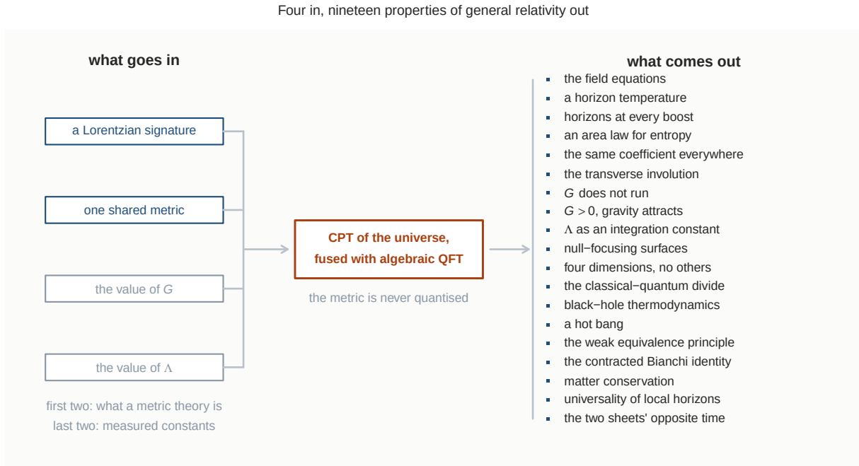
FIG. 1. Inputs and outputs. On the left is everything the fold is given; on the right is everything it returns. Four inputs give nineteen properties of general relativity. Two of the inputs are what writing a metric theory means and two are the measured constants. Full wording of every line is in Appendix A.
