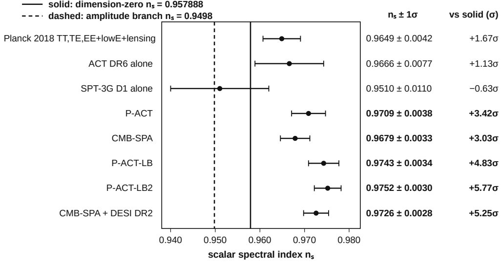
Figure 4. Primordial tilt against 2025–26 CMB data
