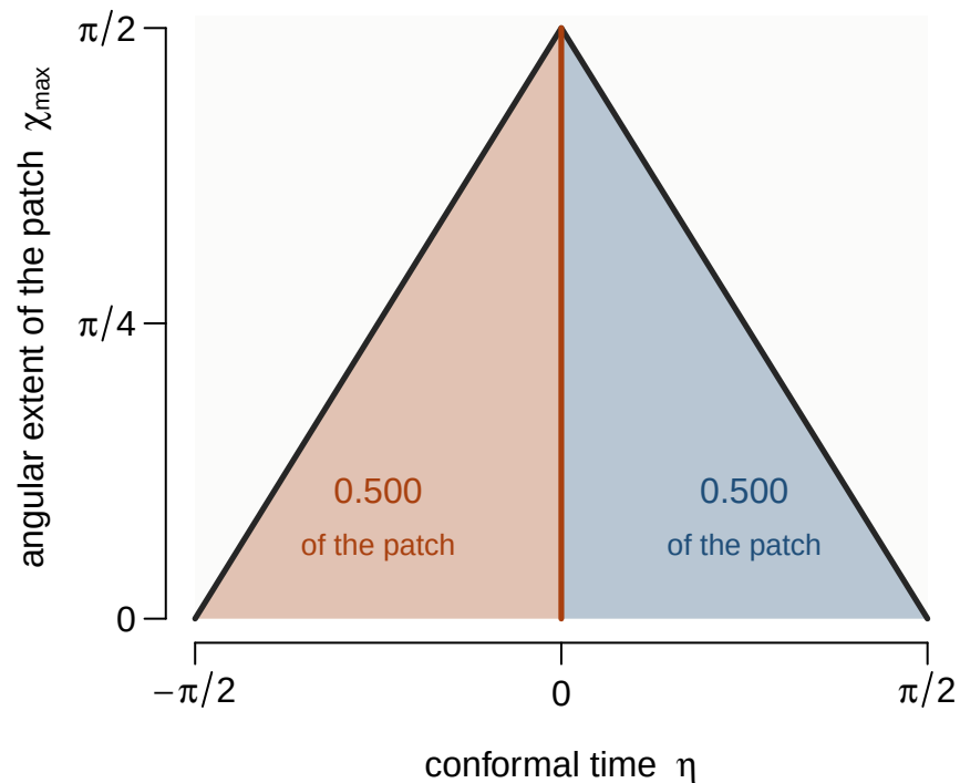
the branch line bisects it, exactly
