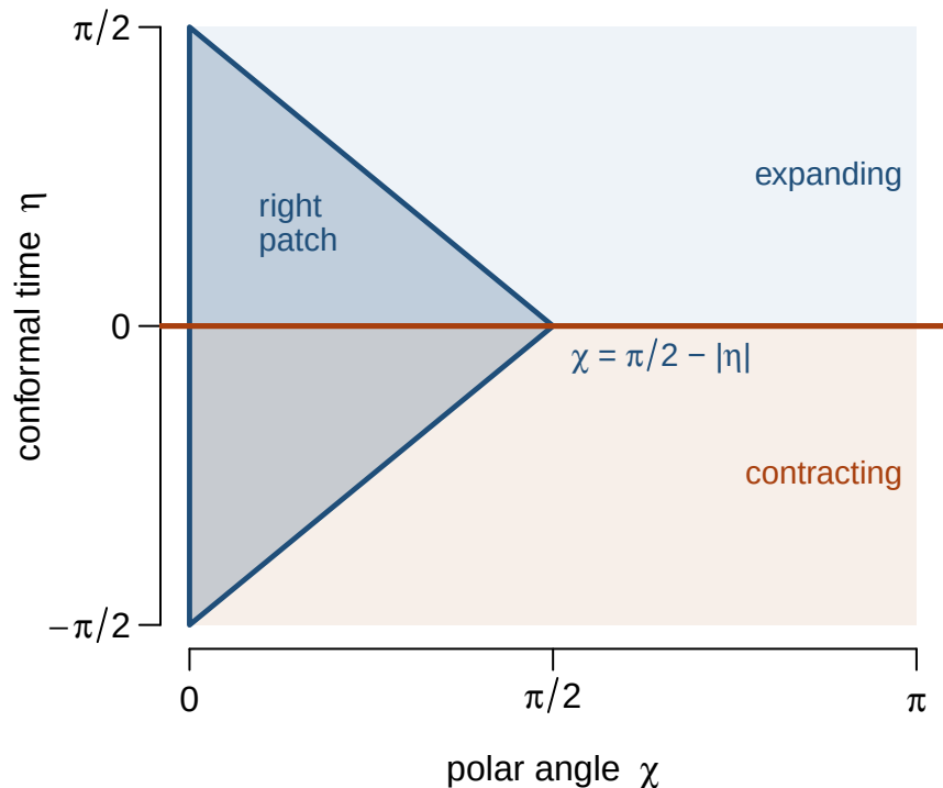
one state, two splittings, drawn together
