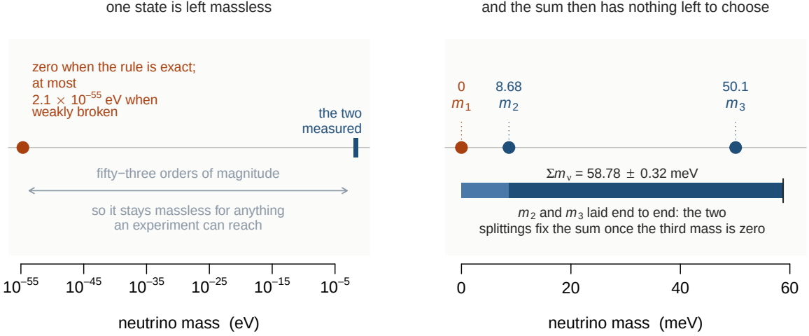
Figure 13: What the rule does to the spectrum. Left, the full range. When the rule is exact the sterile partner’s Yukawa column is forbidden, the light mass matrix has rank at most two, and one light neutrino is exactly massless; the weakly broken version below lifts that zero to at most 2.1 \times 10^{-55} eV for the example lifetime, fifty-three orders of magnitude below the lighter of the two measured splittings. Right, the same spectrum on a linear scale in meV. With m_1 at zero the two splittings fix the sum with nothing left to choose, \Sigma m_\nu = \sqrt{\Delta m_{21}^2} + \sqrt{\Delta m_{31}^2} = 58.78 \pm 0.32 meV for normal ordering, drawn as the two masses laid end to end.
