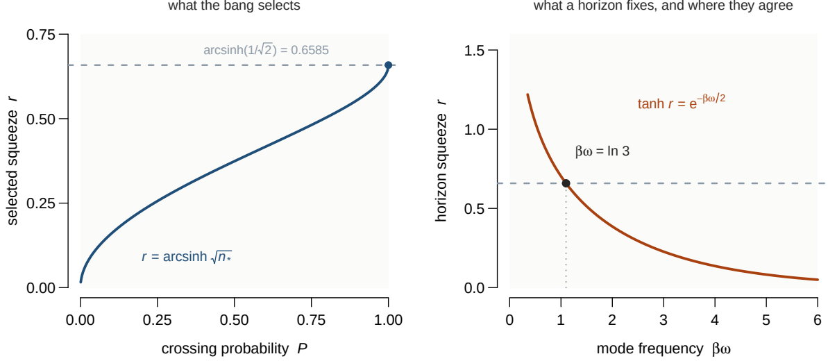
Figure 15: The two ends of the fold, and the one frequency where they agree. Left: what the crossing at the bang selects. Fold-invariance forces half-and-half occupancy, so the pair-block floor is n_*(P) = (1 - \sqrt{1 - P})/2 , and since a squeeze carries \langle N \rangle = \sinh^2 r the selected occupation is a selected squeeze r = \operatorname{arcsinh} \sqrt{n_*} , topping out at \operatorname{arcsinh}(1/\sqrt{2}) = 0.6585 when the crossing is complete. Right: what equilibrium at a bifurcate horizon fixes, the half-period shift making the state a thermofield double with \tanh r = e^{-\beta\omega/2} . The dashed line is the same in both panels, and the horizon curve crosses it at \beta\omega = \ln 3 exactly, to machine zero. The reason is that both ends are statements about one half: \Theta -invariance caps the crossing at half occupancy, a horizon mode is half occupied where the Bose factor is one half, and that is e^{\beta\omega} = 3 . The curves meet because they say the same thing.
