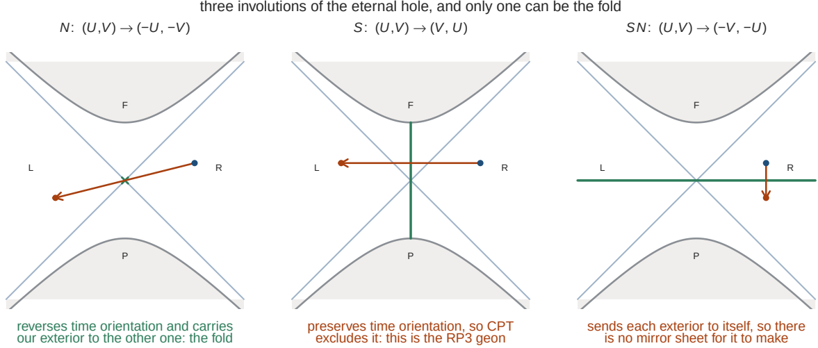
Figure 16: The classification, and what separates the three. In Kruskal coordinates T = (U + V)/2 and X = (V - U)/2 the survivors of the squaring are the point reflection through the origin, the mirror in the vertical axis and the mirror in the horizontal one. Shaded, the singularities; thin diagonals, the horizons; green, each map's fixed set, which is a point for N and a line for the other two. The blue dot is a point of our exterior R and the orange one is its image. S carries R to L but preserves time orientation, so a CPT map cannot be it; it is the \mathbb{RP}^3 geon. SN reverses time orientation but sends each exterior to itself, so it offers no mirror sheet at all, and the contact it would describe would sit where we can look. N does both things the fold needs and, unlike the swaps, admits no boost freedom to fix afterwards. The script checks that all three preserve UV and square to the identity, and that a fourth map does neither.
