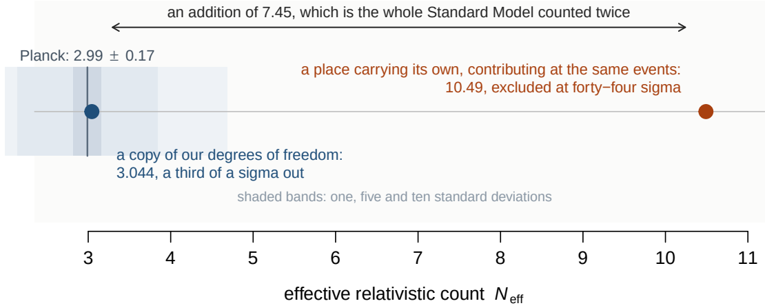
Figure 14: The arithmetic that looks decisive. Writing \rho_{\text{rad}} = \rho_\gamma(1 + 0.2271N_{\text{eff}}) with 0.2271 = (7/8)(4/11)^{4/3} , the Standard Model’s 1.691\rho_\gamma duplicated is an addition of 7.45 in N_{\text{eff}} units, which is the whole Standard Model counted twice. Against Planck’s 2.99 \pm 0.17 the copy reading sits a third of a standard deviation away and the place reading forty-four. The paper does not claim that exclusion. Duplicating the density requires the two sheets’ stress-energy to add at the same events, and the fold puts them at different ones, which is the same fact that makes the silence of Section 1 a theorem. Both readings therefore predict the left-hand point and Planck does not separate them. The figure is here to show how large a gap the argument would have carried had it applied, and how little it gives without co-location.
