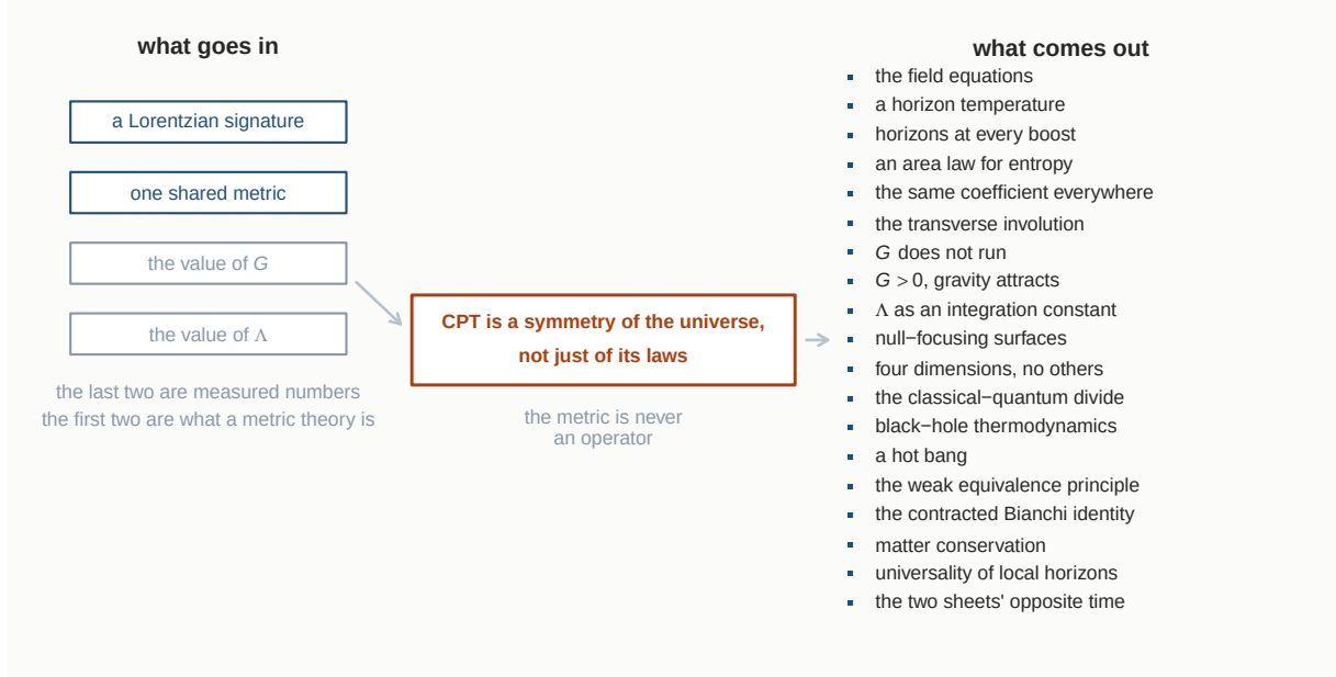
Figure 5. The ledger. On the left is everything the fold is given: a Lorentzian signature and one metric carrying both the fold's horizons and a covariant matter action, which between them are what writing a metric theory means, and the measured values of G and \Lambda . In the middle is the single postulate, that CPT is a symmetry of the universe and not only of its laws. On the right are the nineteen properties of general relativity that follow, the metric staying a fixed background throughout. The dependency graph behind the two columns is acyclic and no path from the field equations reaches general relativity or Bekenstein-Hawking
