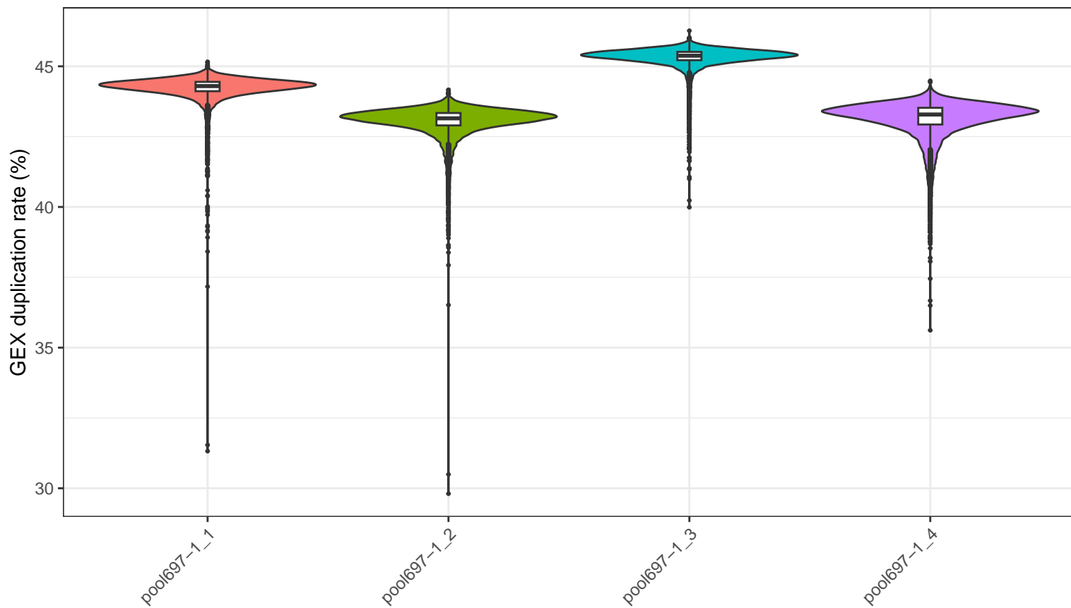
Exonic read duplication rate
