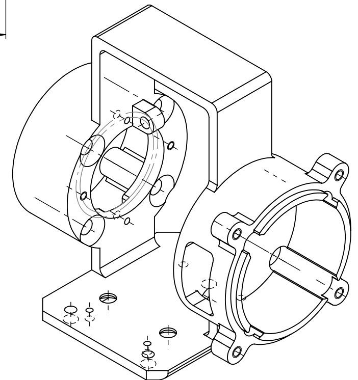
Isometric View
