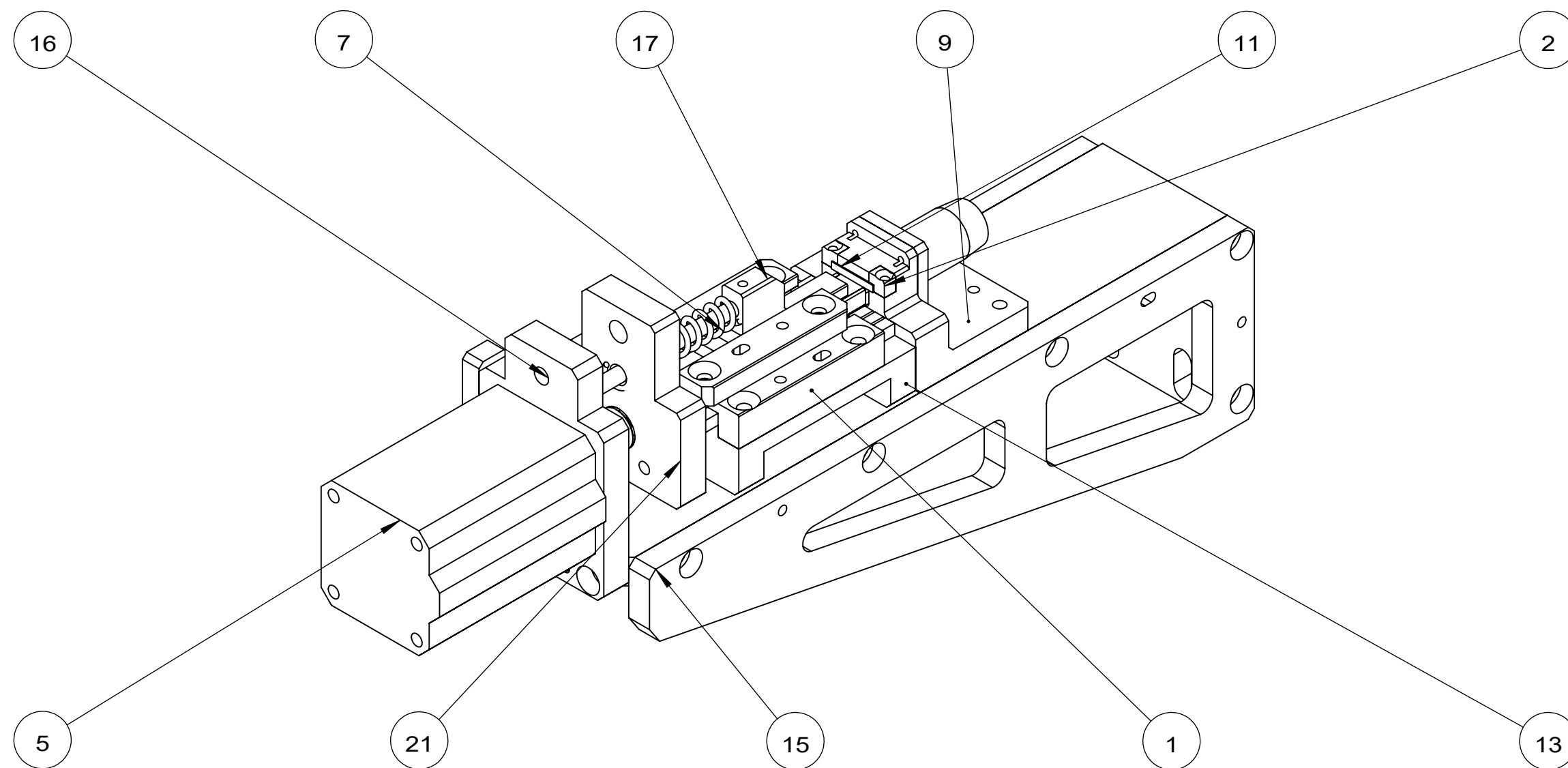
ISOMETRIC ASSEMBLY VIEW
