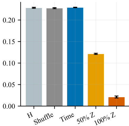
weather
