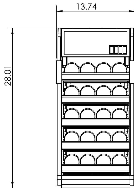
Countertop Full compression 5 shelves 20 facings
