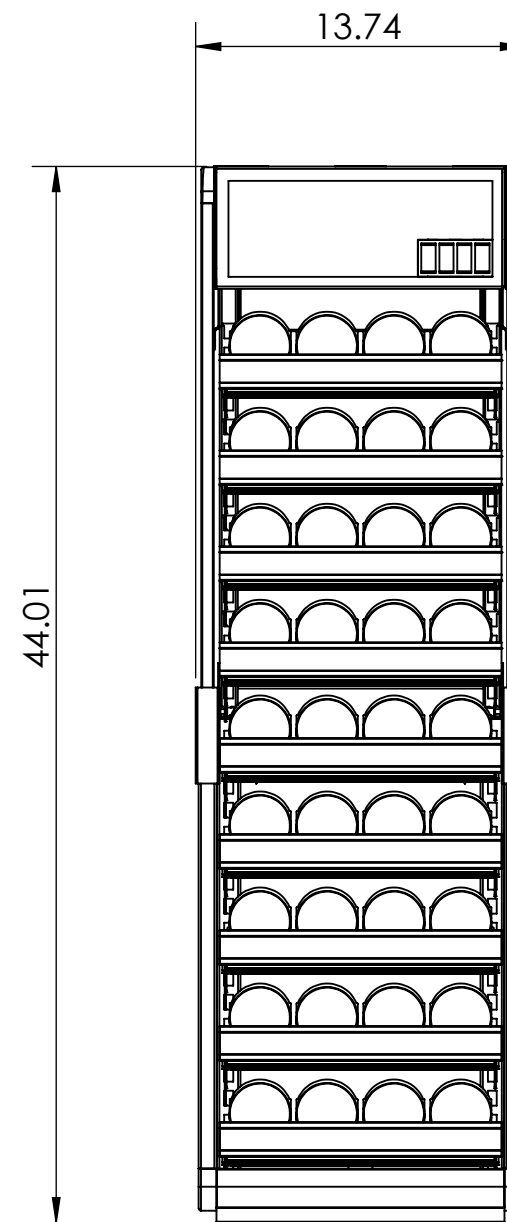
Countertop Full expansion 9 shelves 36 facings
