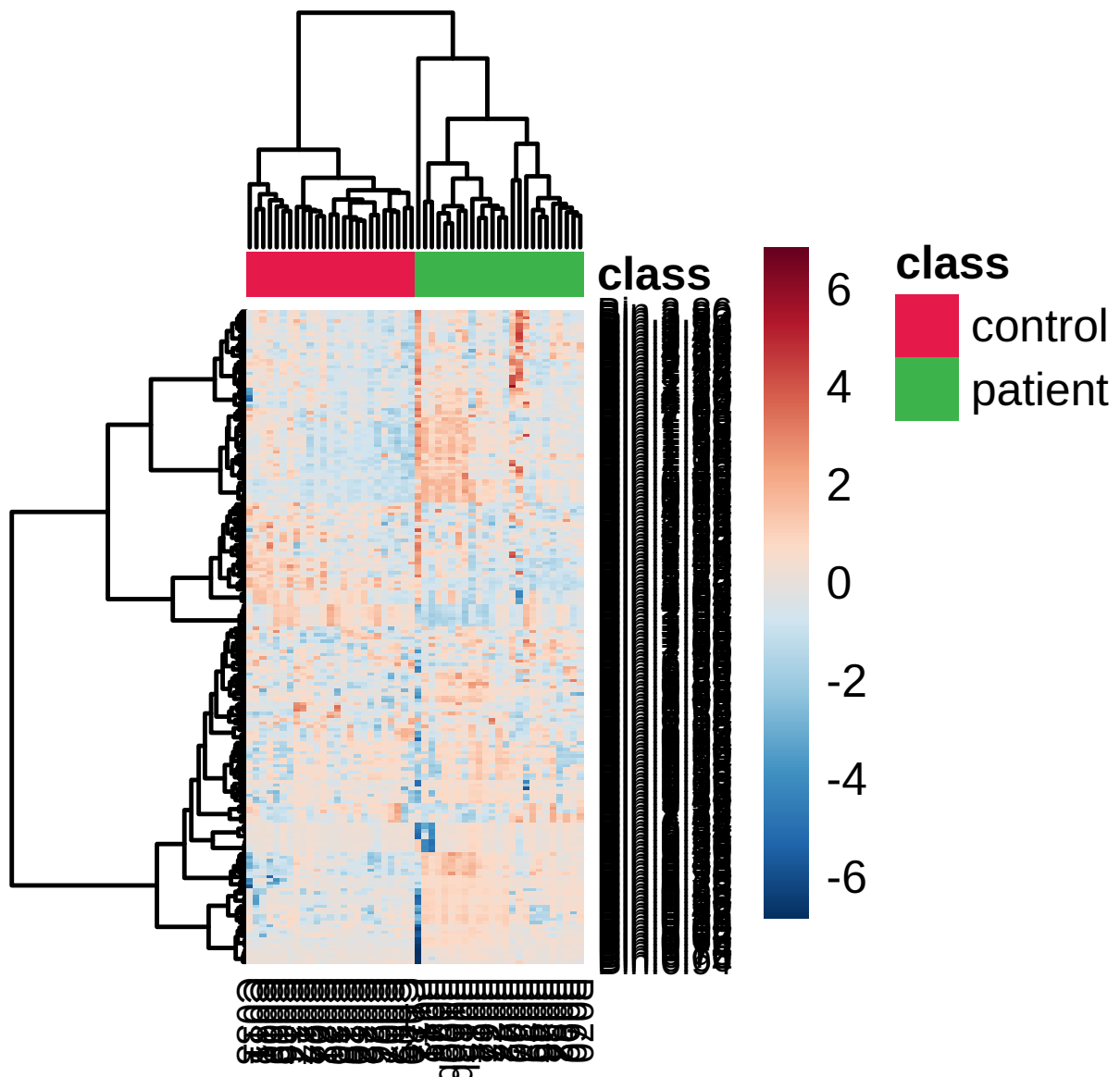
Figure 12: Clustering result shown as heatmap (distance measure using euclidean , and clustering algorithm using ward.D ).
