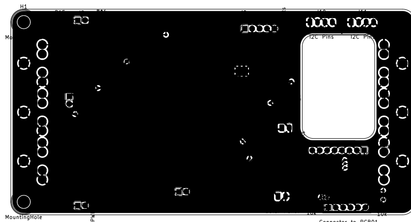
Connector to PCB01
