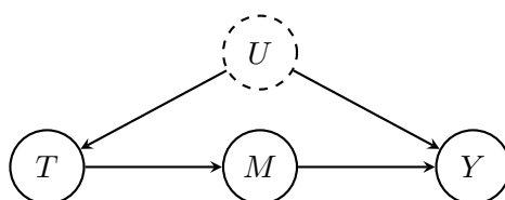
Figure 3: Frontdoor DAG with mediator M and unobserved U .
