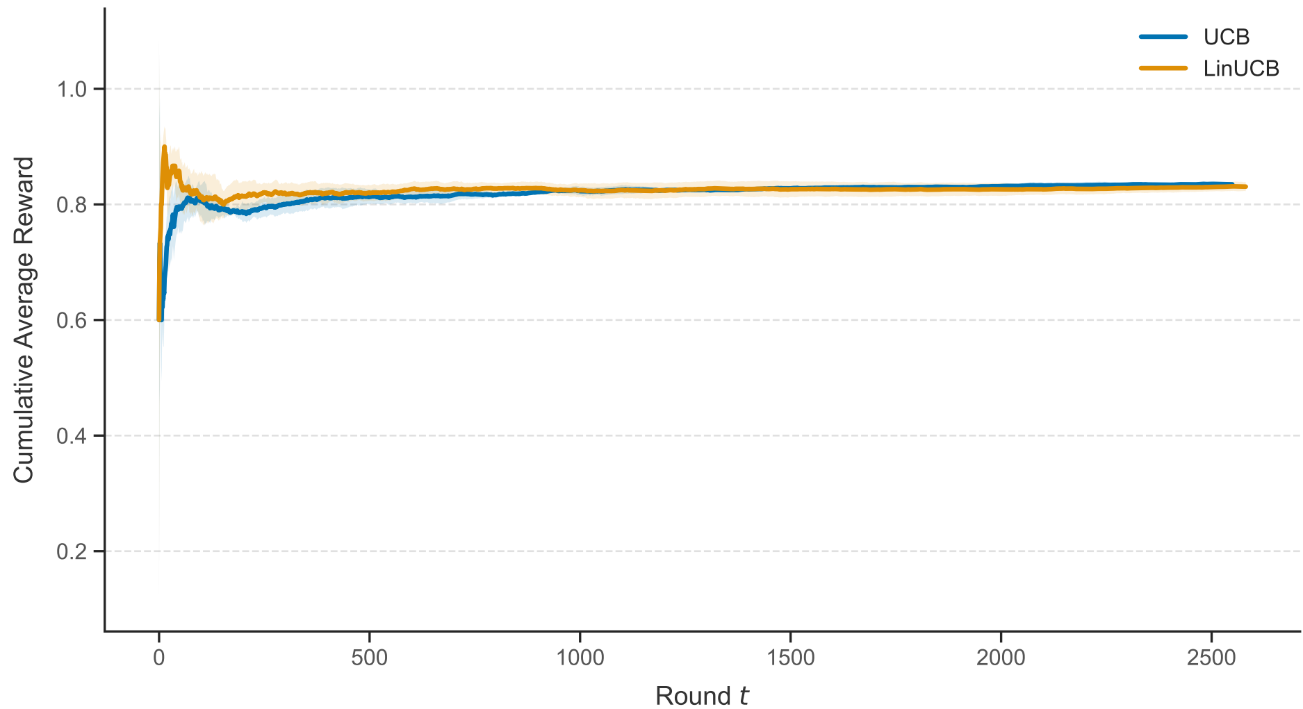
MovieLens 1M Offline Replay Evaluation
