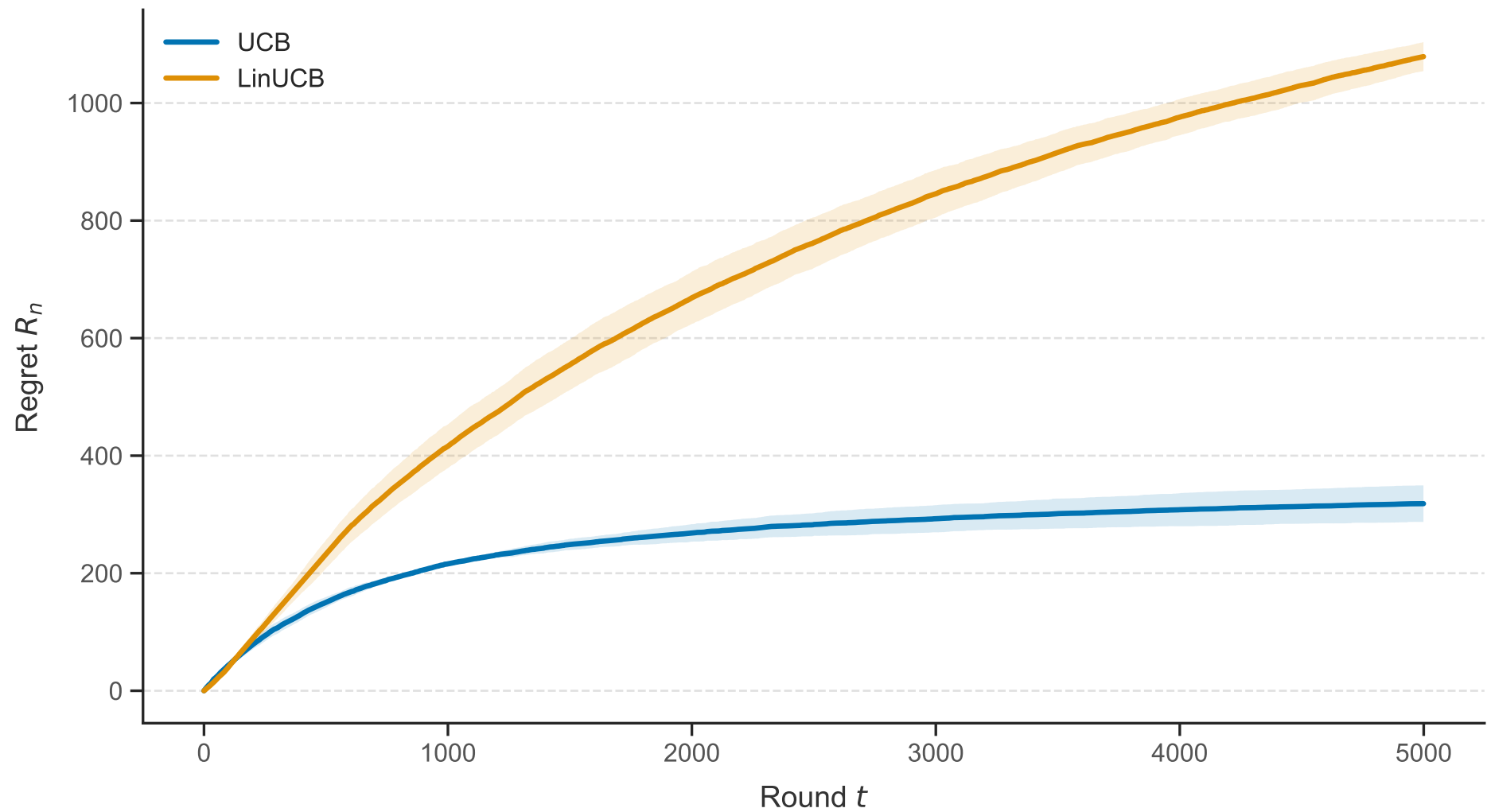
Regret on Non-Contextual Data
