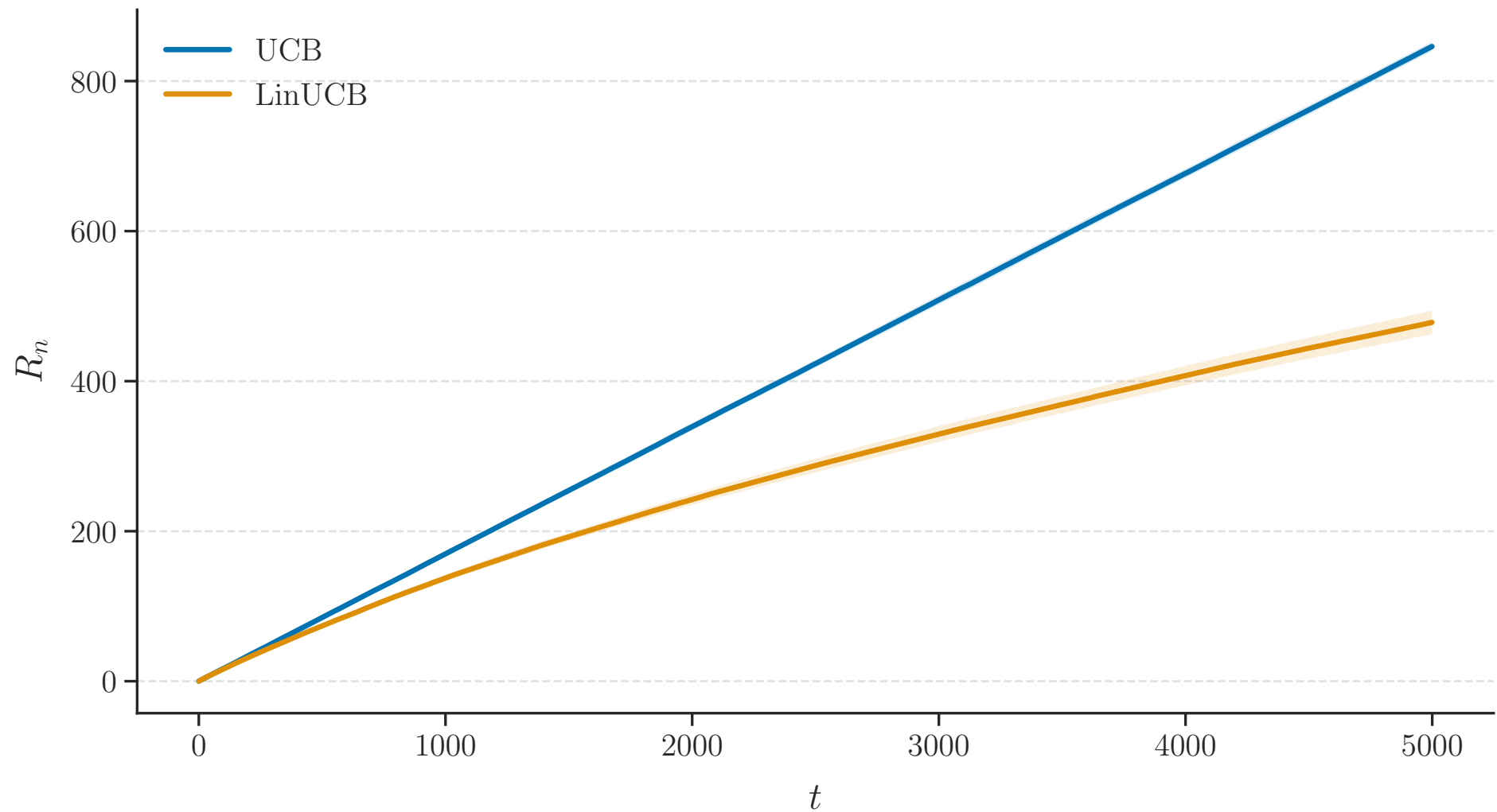
Regret on Contextual Data
