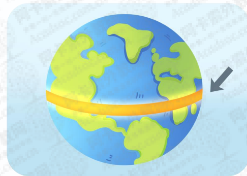
equator
