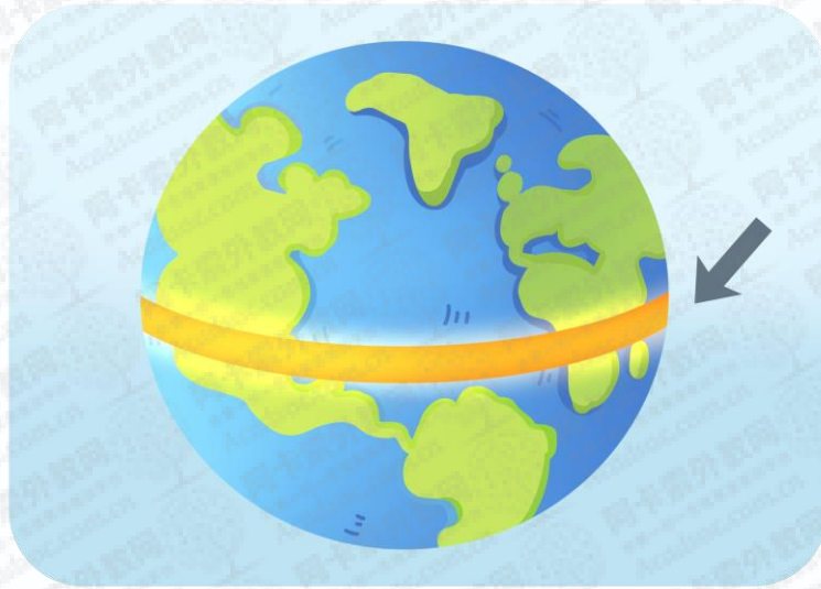
equator
