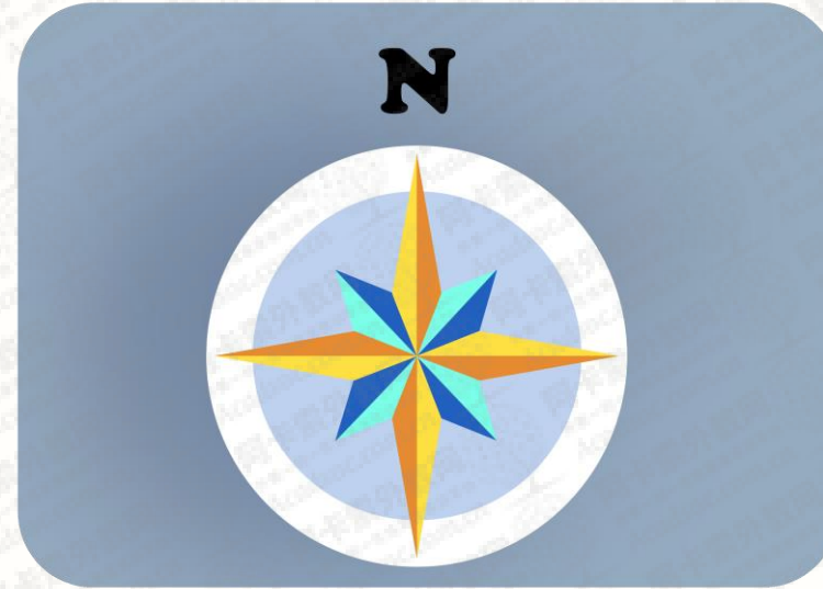
north
