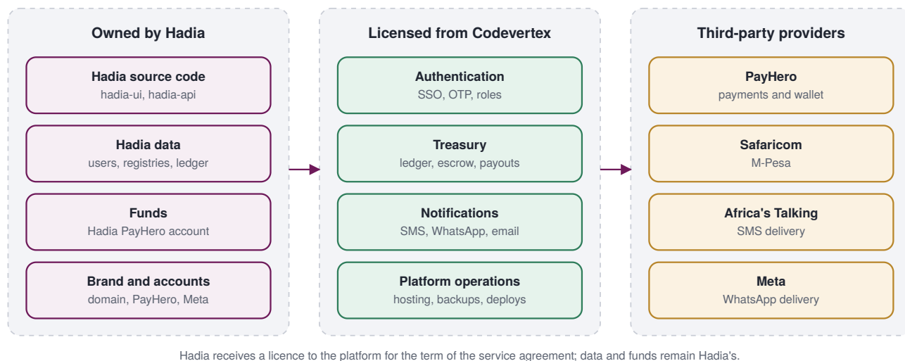
Figure 15. Ownership boundaries
