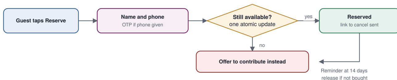
Figure 10. Item reservation
