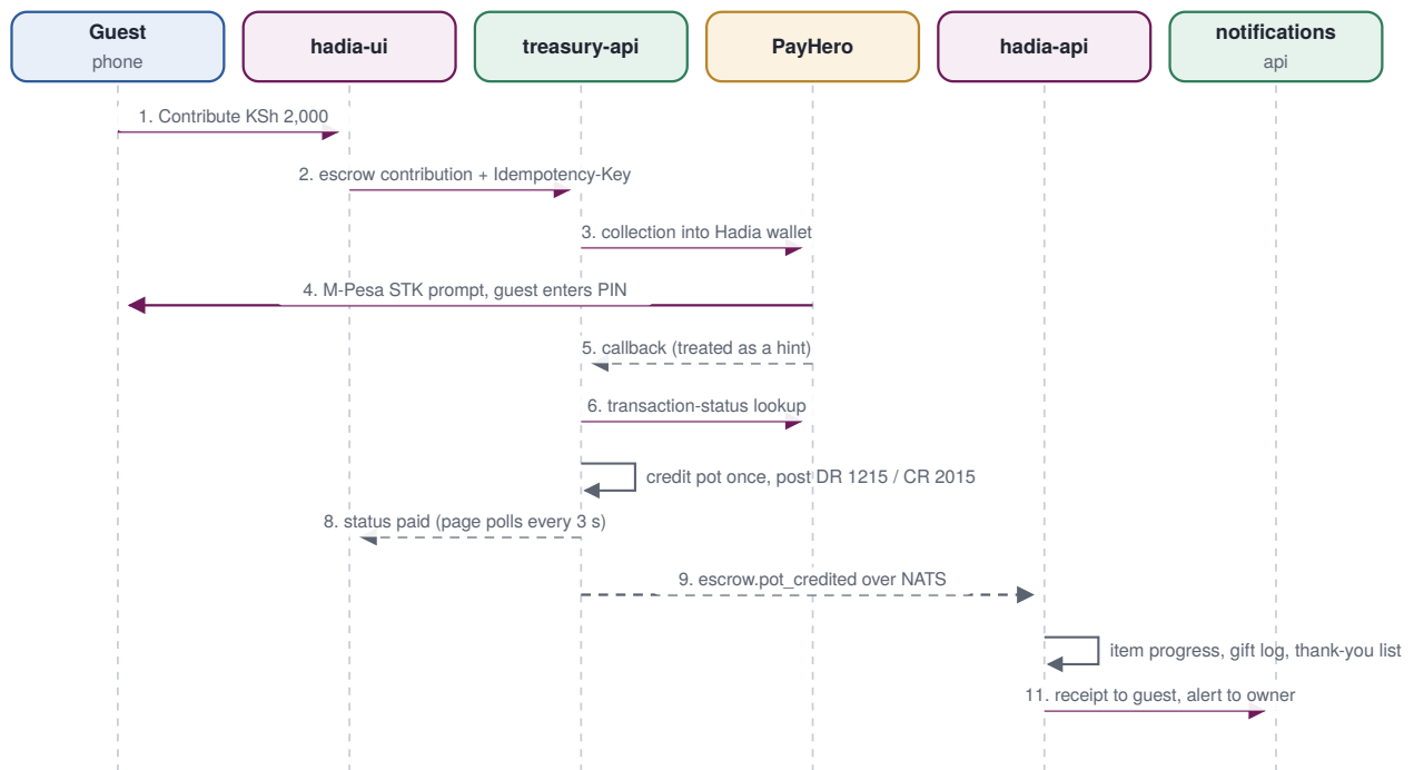
Figure 11. Cash contribution sequence
