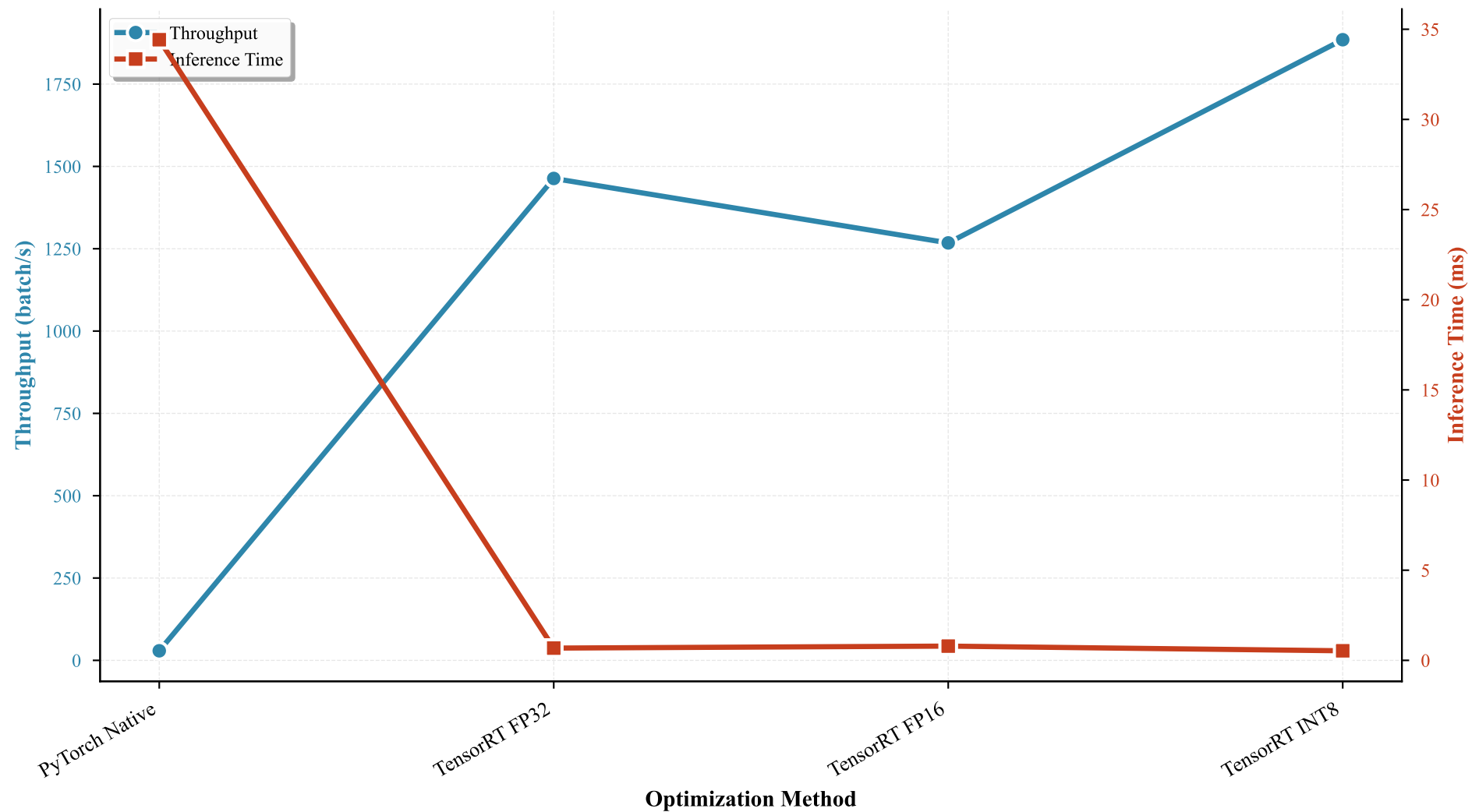
Performance Comparison: Throughput vs. Inference Time
