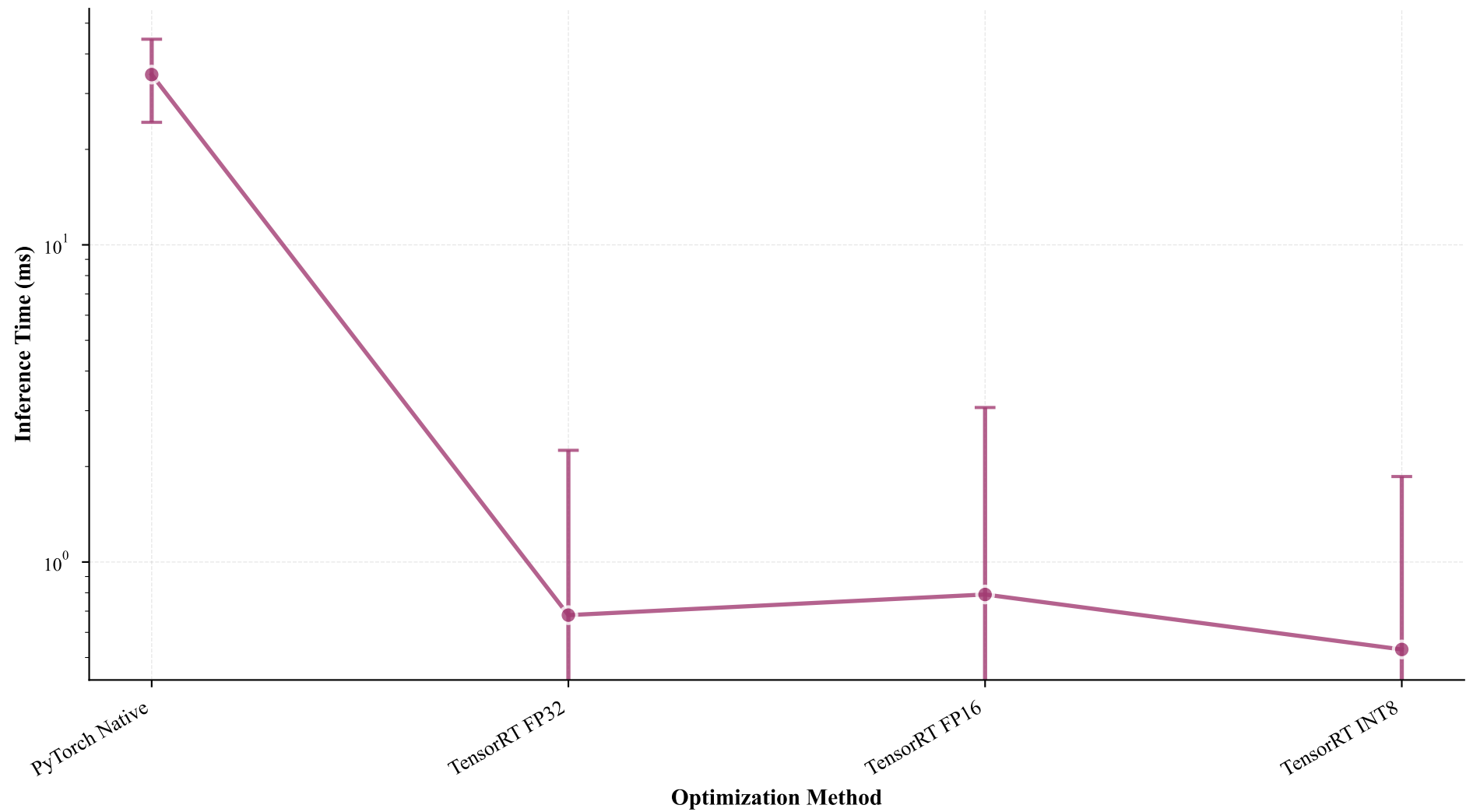
Inference Time with Standard Deviation
