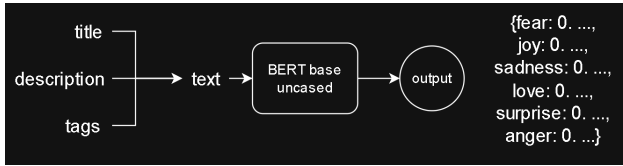
Figure 2. NLP
