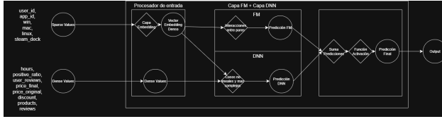
Figure 1. DeepFM
