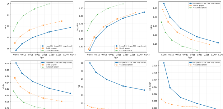
AEIC-SE: rate-distortion-perception on ImageNet-1k vs. paper benchmarks
