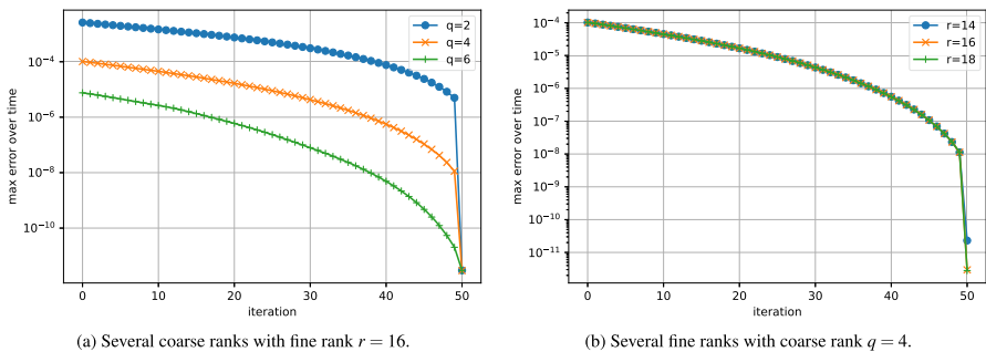
Fig. 6 Convergence of the error of low-rank Parareal for the parametric cookie problem (32). Influence of the coarse and fine ranks
