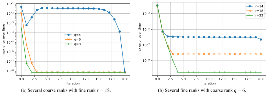
Fig. 8 Convergence of the error of low-rank Parareal for the Riccati problem (33). Influence of the coarse and fine ranks
