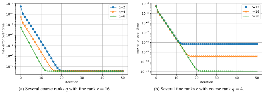
Fig. 3 Convergence of the error of low-rank Parareal for the Lyapunov ODE (27) with n = 100 and T = 2.0 . Influence of the coarse and fine ranks
