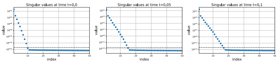
Fig. 5 Singular values of the solution over time of the parametric cookie problem (32)
