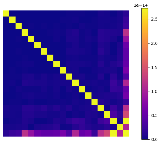
Householder
