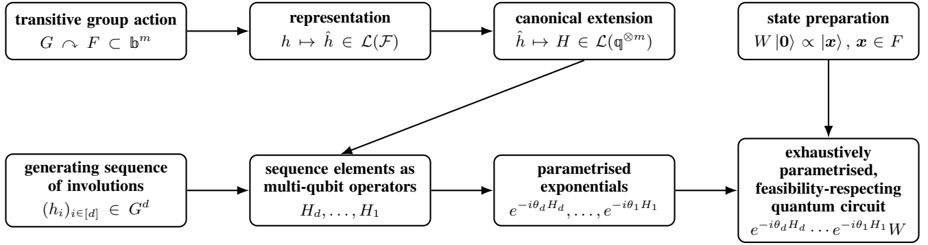
Fig. 2. Abstract pipeline for constructing an exhaustively parametrised, feasibility-respecting quantum circuit from a transitive group action on the feasible set F \subset \mathbb{B}^m . Central to this construction is the existence of a generating sequence of involutions, whose elements can be represented as m -qubit operators. Exponentiating these operators, introducing real parameters in the exponent, and prepending the state preparation of some feasible computational basis state |x\rangle , completes the construction.
