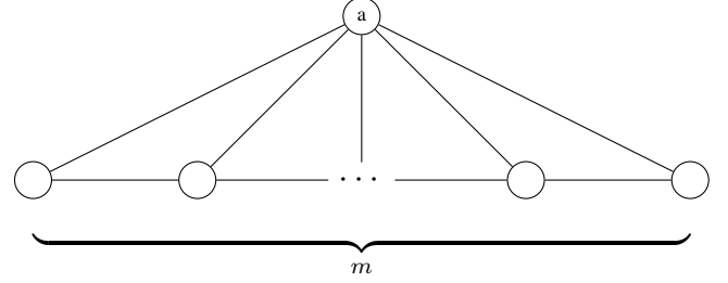
Fig. 4. Qubit connectivity required for implementing the exhaustively parametrised quantum circuit based on the bubble sort sequence. The m data qubits, encoding the TSP solutions, can be aligned on a chain. The ancilla qubit, serving as control for the Fredkin gates, has to be connected to all m data qubits. Alternatively, one can introduce m - 1 ancilla qubits, each connected to two contiguous data qubits.
