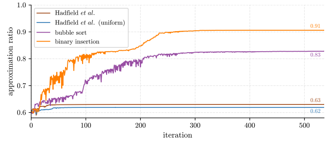
Fig. 5. Approximation ratios obtained after each COBYLA iteration, using different parametrised quantum circuits on a 9-city TSP instance. The QAOA with Hadfield et al. ’s mixers—initialised either in a single computational basis state or in the uniform superposition of all feasible states—was not able to significantly improve the initial approximation ratio. In contrast, the exhaustively parametrised circuit based on bubble sort pushed the initial ratio of \approx 0.60 to 0.83, while the binary insertion sequence even reached 0.91. Not depicted here: the bubble sort-inspired approach ran for 2300 steps without significant improvement, whereas the binary insertion and single-basis-state QAOA variants terminated after roughly 600 steps, and the uniform-initialisation QAOA already after roughly 150.
