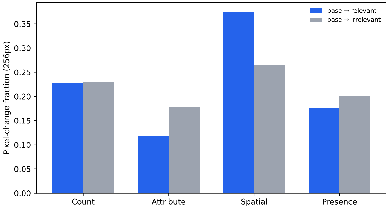
Edit magnitude (not LPIPS; scene masks unavailable)
