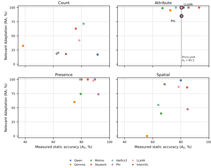
Figure 3: Measured static accuracy versus RA by factor. The Attribute panel highlights the Phi-LLaVA exact tie at 80.5% static accuracy and their 84.95% versus 100.00% RA values.
